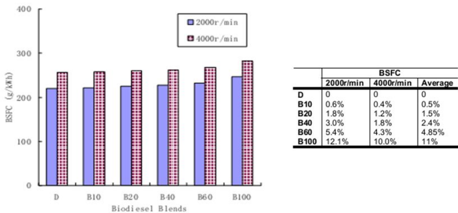
Figure 8. BSFC of different biodiesel blends at two speeds [33]
