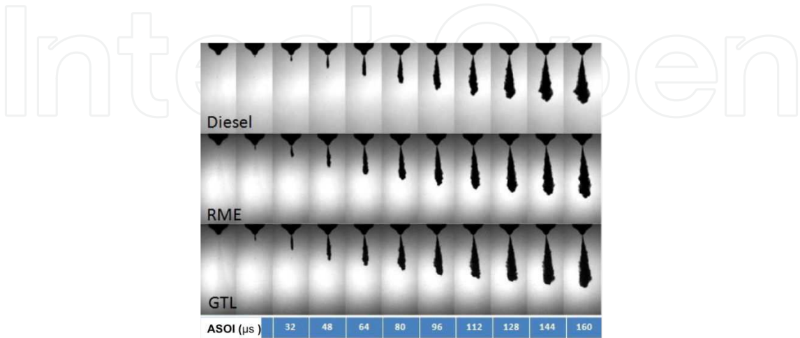
Figure 4. Sequence of spray images in a single time-resolved ULSD spray ( P_{inj} =120 MPa, P_{amb} =3.0 MPa and t_{dur} =1.5 ms)
