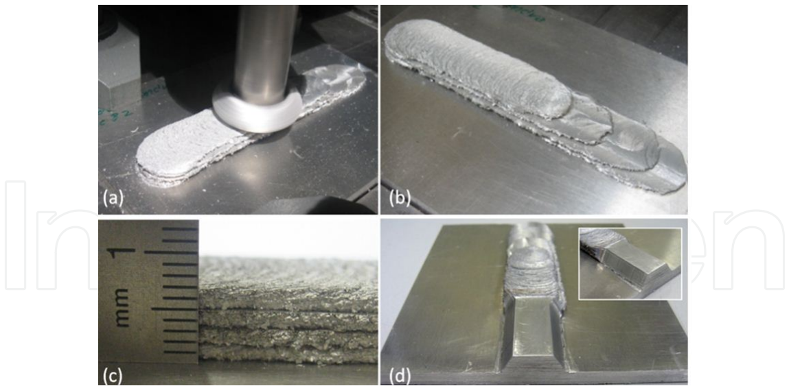
Figure 8. Build-up by friction surfacing. a) Successive deposition; b) Bulk produced from four overlapped passes; c) Detail of final thickness achieved; d) Milling of linear rail.
