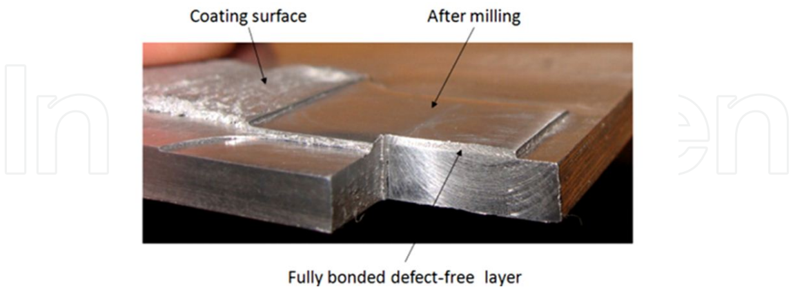
Figure 7. Surface finish by milling. FS of AA6082-T6 over AA7178-T6.
