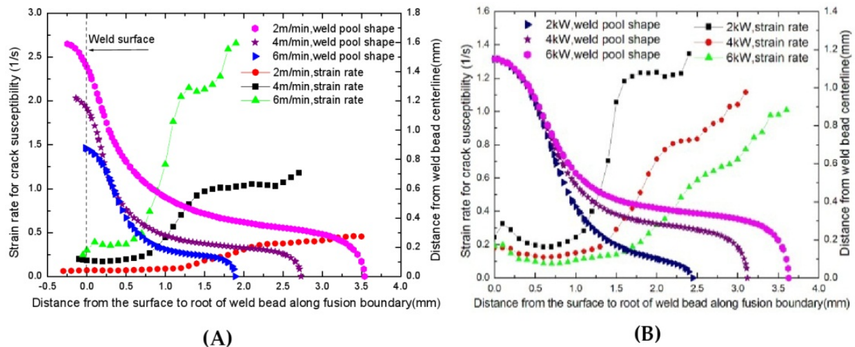
Figure 11. Correlation between the shape of weld pool and strain rate with various welding conditions for laser-arc hybrid welding, (A) variation of welding speed, (B) variation of laser power (Gao & Ojo, 2012b)
