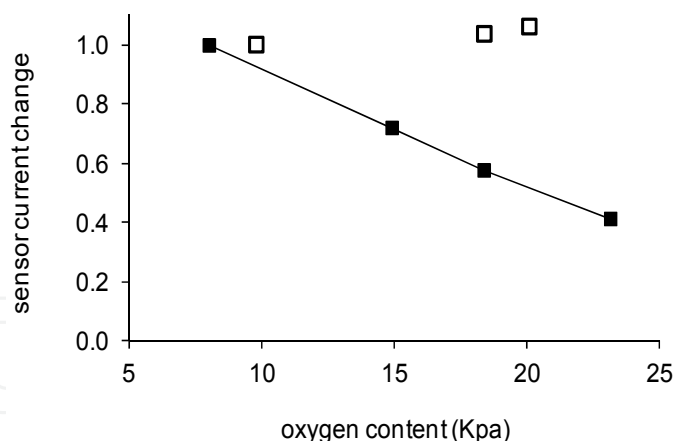
Figure 12. Effect of oxygen content on current response to 5 mM glucose in 0.01M pH7.4 PBS for screen-printed electrodes containing FAD-GDH (□) and GOx (■), tested by using an Ag/AgCl reference electrode and a platinum counter electrode
