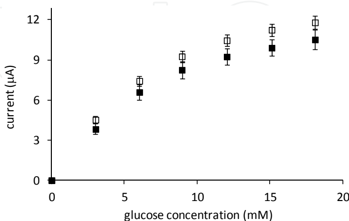
Figure 13. Calibration plots for screen-printed electrodes before (□) and after (■) 25 KGy e-beam sterilization, tested in 0.01M pH7.4 PBS by using an Ag/AgCl reference electrode and a platinum counter electrode, the error bars are first standard deviation of 7 electrodes
