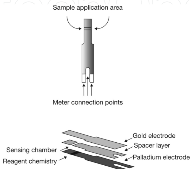
Figure 7. Architecture of the OneTouch Verio glucose test strip. The test strip incorporates gold and palladium electrodes that are orientated in a cofacial manner. The dimensions of the two electrodes are defined and controlled during the manufacturing process by a die-punch process. The electrodes are separated from each other by a thin plastic spacer that has a nominal thickness of 95 \mu\text{m} . The glucose-sensitive reagents, citraconate buffer salts, potassium ferricyanide mediator, and flavoprotein glucose dehydrogenase, are laid down on the "bottom" palladium electrode. The user can apply blood to the test strip either from the right hand side or the left hand side. The glucose level is reported within 5 seconds of the start of the test procedure.
