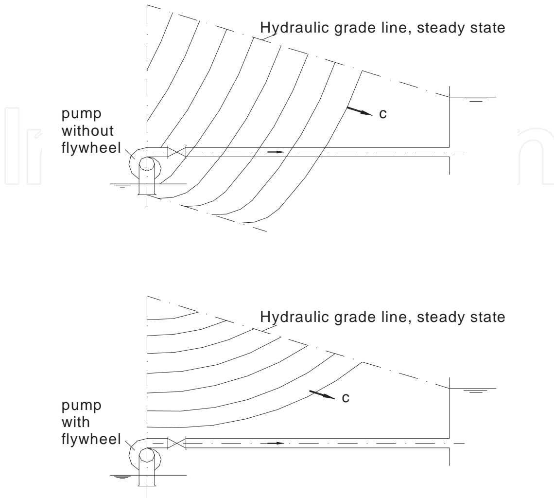
Figure 9. Effect of flywheel on transient pressure after power failure in the pumping station
