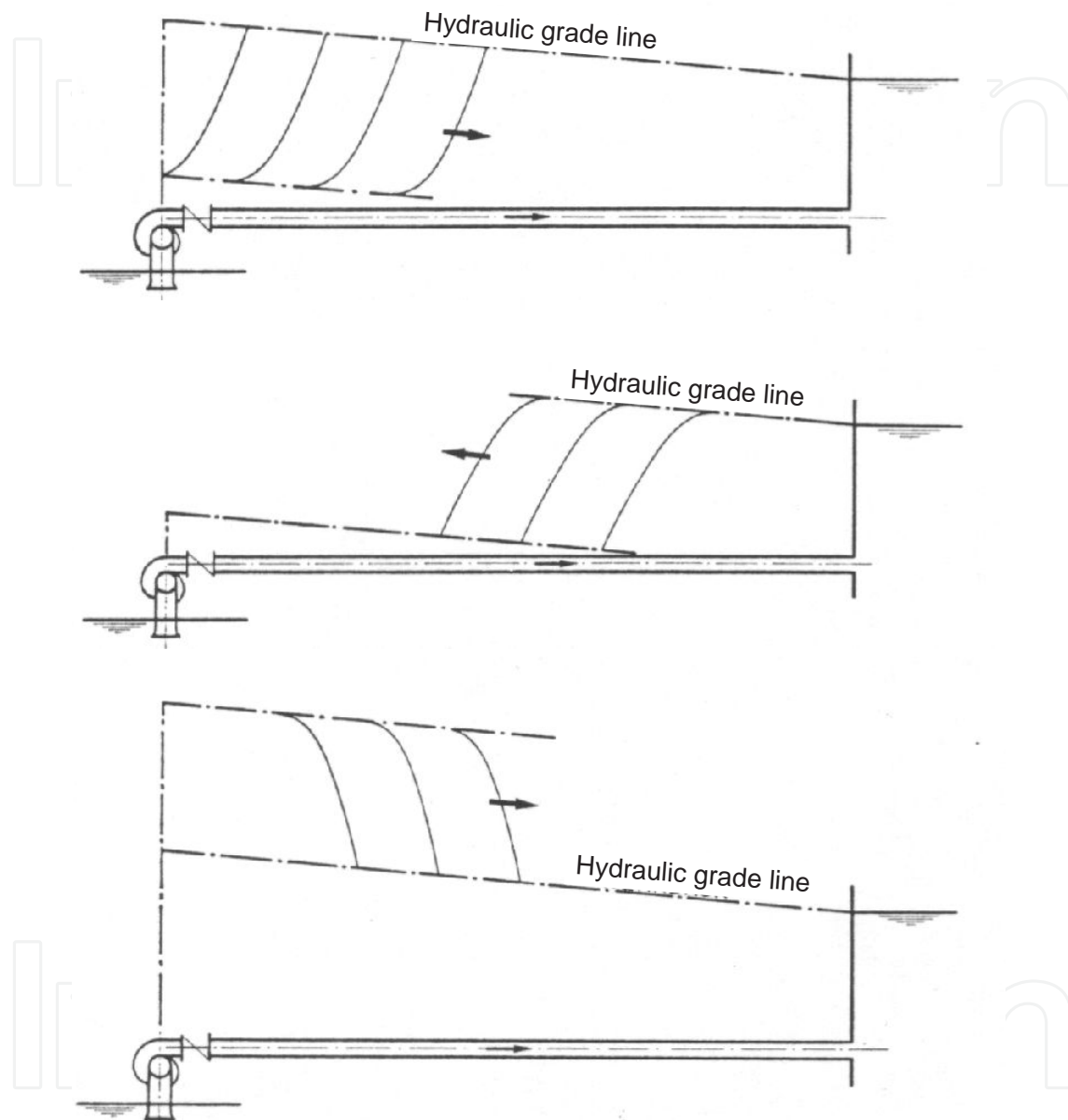
Figure 4. Pressure wave propagation following a pump trip
