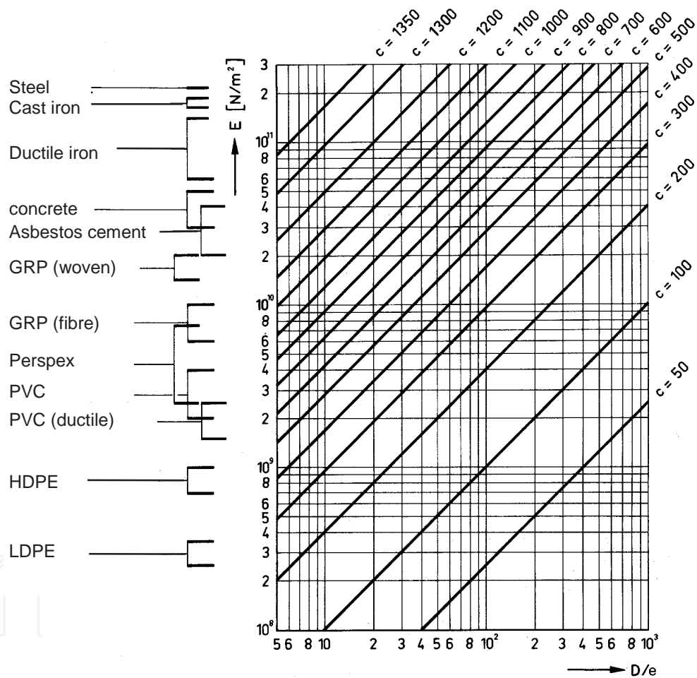
Figure 3. Graph of acoustic wave speed in water pipelines in relation to pipe material ( E ) and wall thickness ( D/e ).
