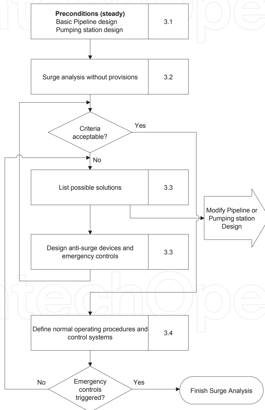
Figure 2. Integrated design for pressure transients and controls.
