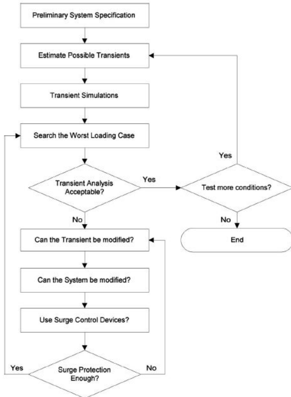
Figure 1. Pressure Transient design (Jung and Karney 2009).
