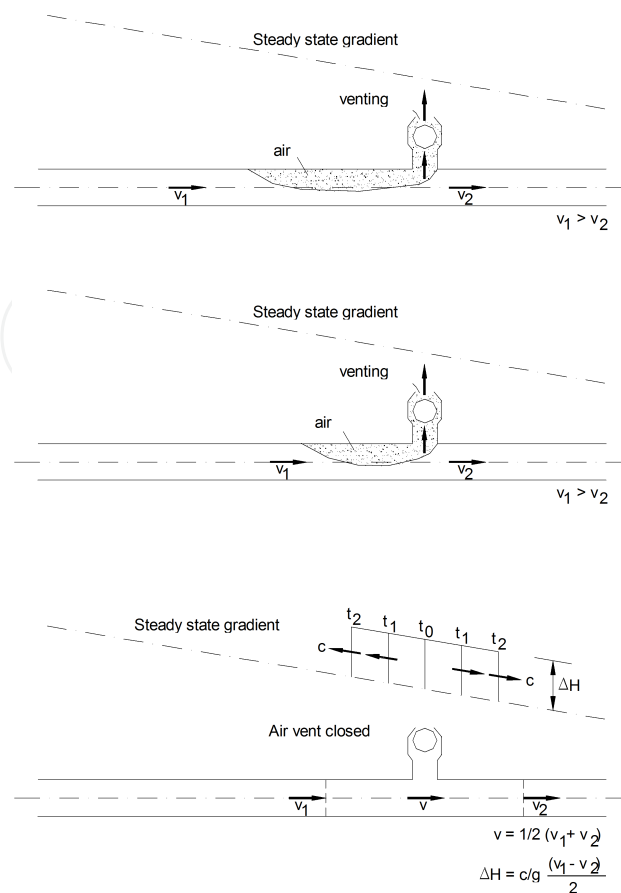
Figure 10. Pressure shock due to air valve slam.
