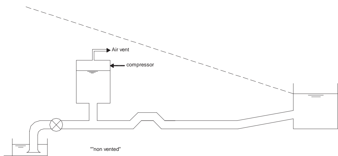
Figure 7. Non-aerated surge vessel
