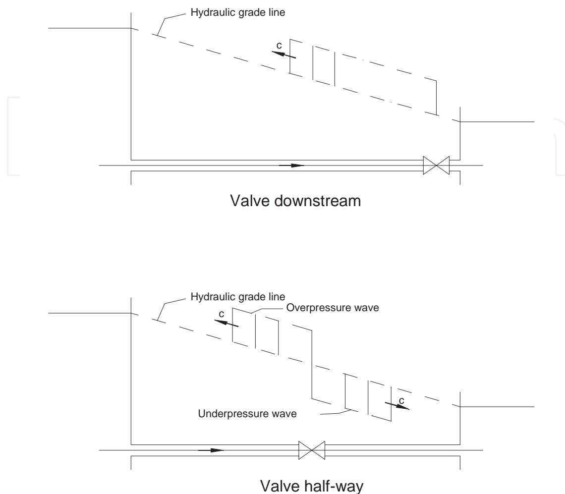
Figure 5. Pressure wave propagation following valve closure
