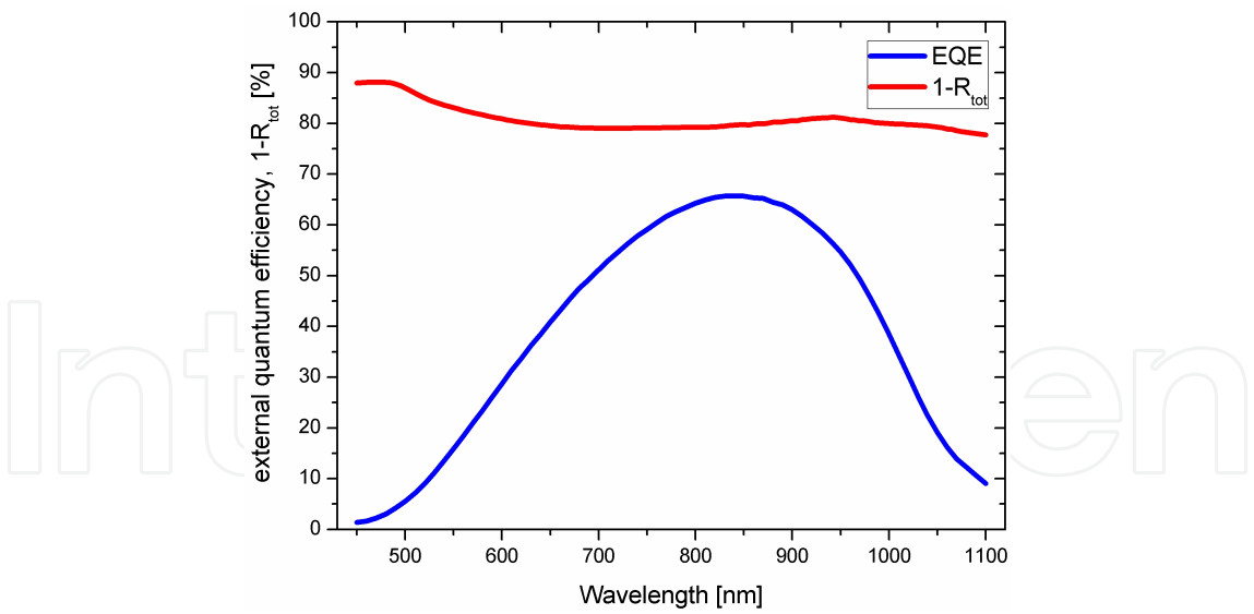
Figure 10. Absorption ( 1-R_{\text{tot}} ) and EQE of a SiNW-based solar cell prototype.
