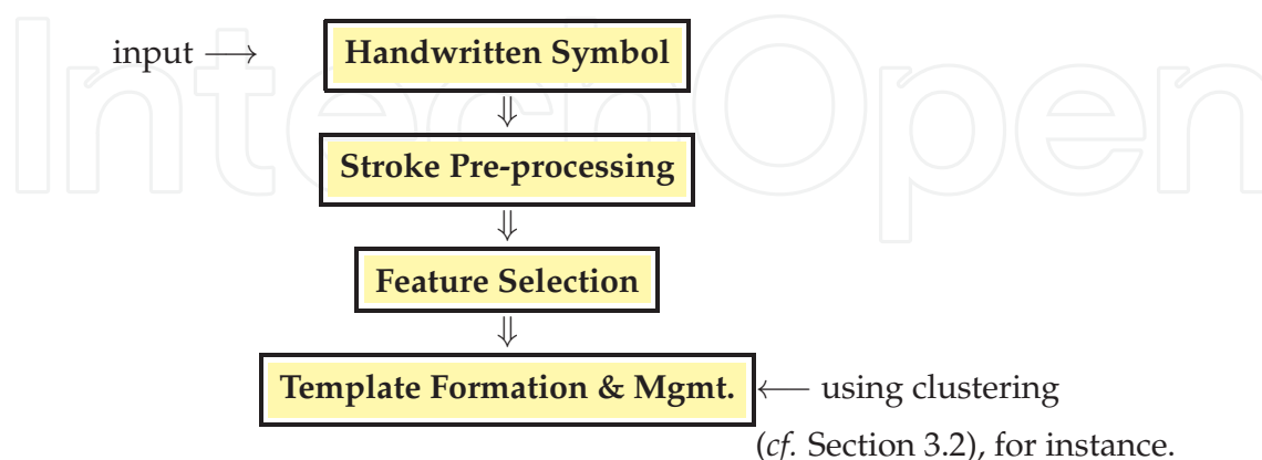
Figure 3. Learning strokes from the handwritten symbols. In this illustration, we present a basic concept to form template via clustering of features of the strokes immediately after they are pre-processed.
