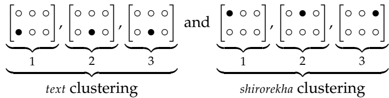
Figure 9. Clustering technique for each class. Stroke clustering is based on the relative positioning. As a consequence, we have three clustering blocks for text strokes and remaining three for shirorekha .
