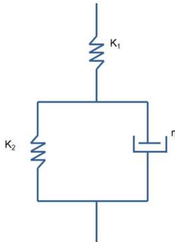
Figure 4. A schematic representation of standard solid model used to determine viscoelastic parameters. Adapted from [19] with permission.
