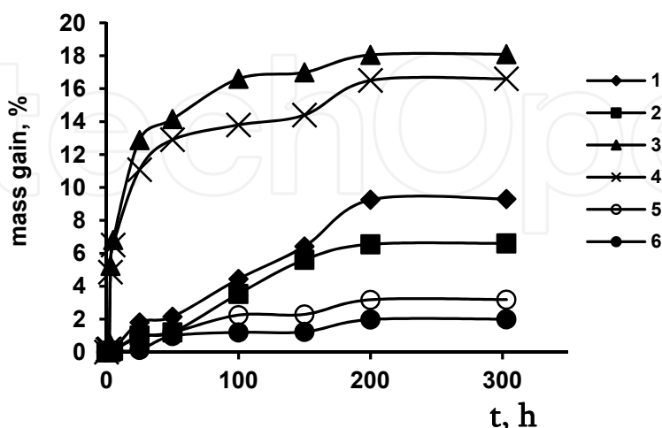
Figure 8. Degree of the mass gain of solutions as a function of the process duration t . sample №2: dehydrated zeolite 1 – toluene; 3- acetone; 5- carbon tetrachloride. air-dry zeolite 2- toluene; 4- acetone; 6- carbon tetrachloride.
