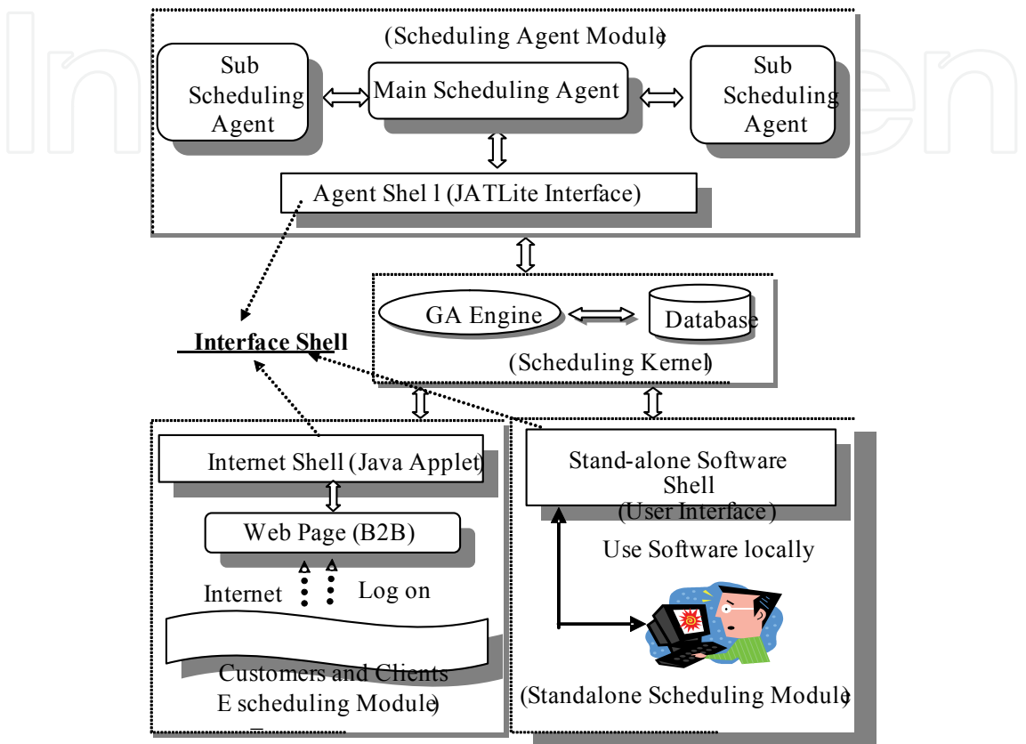
Figure 5. Scheduling agent
