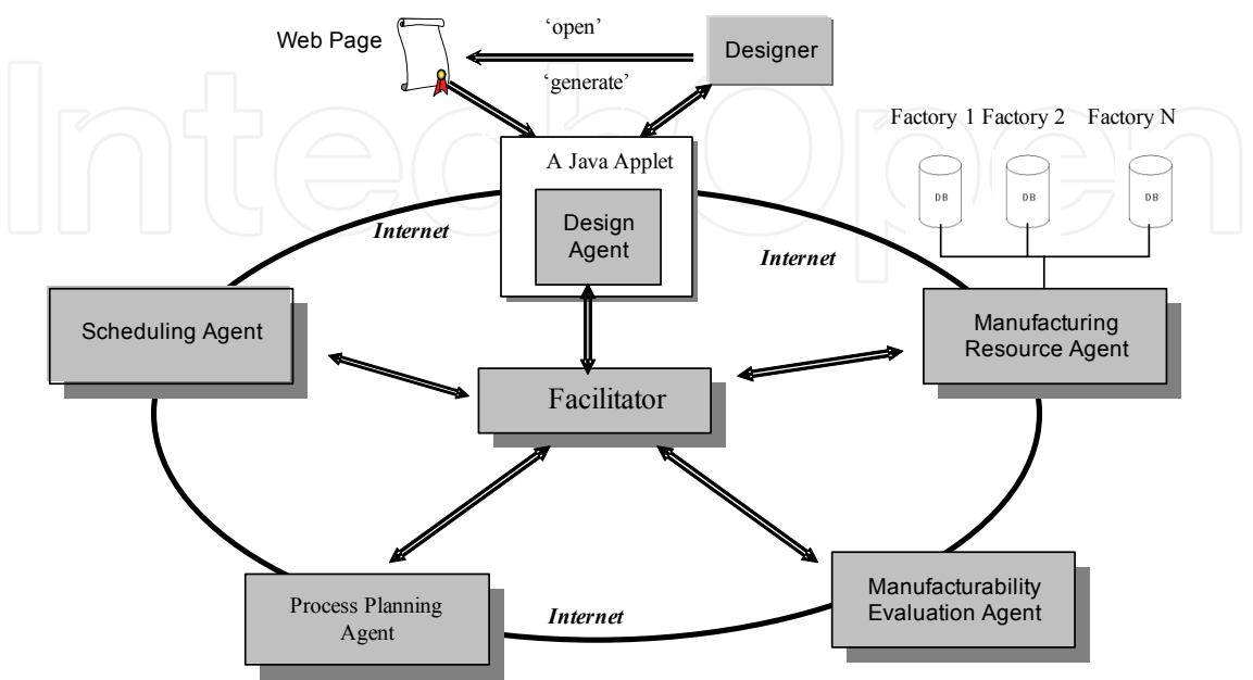
Figure 3. System architecture
