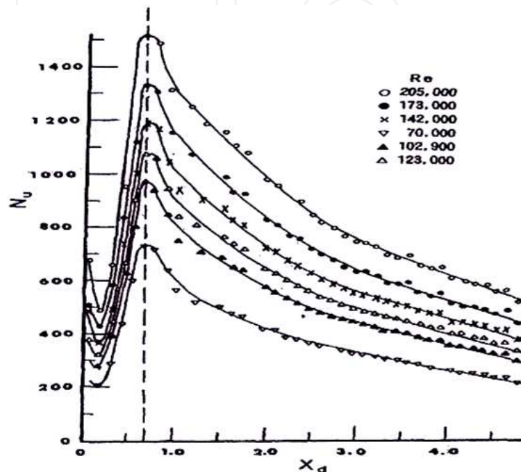
Figure 3. Local Nusselt number distribution.
