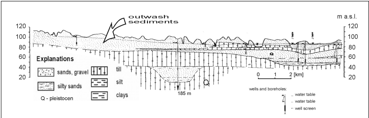
Figure 3. Geologic cross-section along line A-A' in figure 4.
