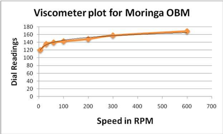
Figure 8. Viscometer Plot for Moringa OBM
