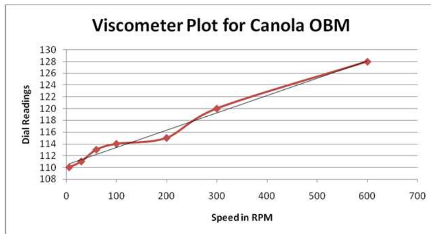
Figure 10. Viscometer Plot for Canola OBM
