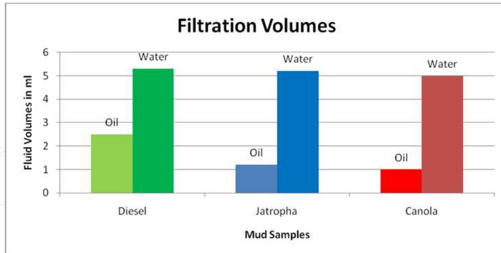
Figure 13. Filtration Volumes for Diesel, Jatropha and Canola OBM's
