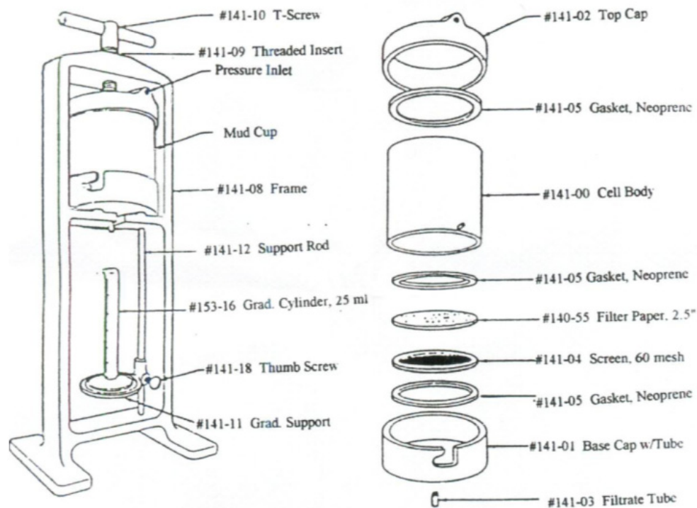
Figure 5. API Filter Press
