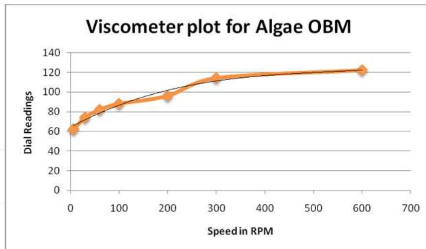
Figure 9. Viscometer Plot for algae OBM
