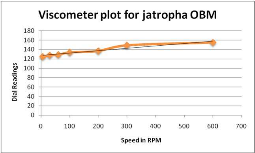
Figure 7. Viscometer Plot for Jatropha OBM
