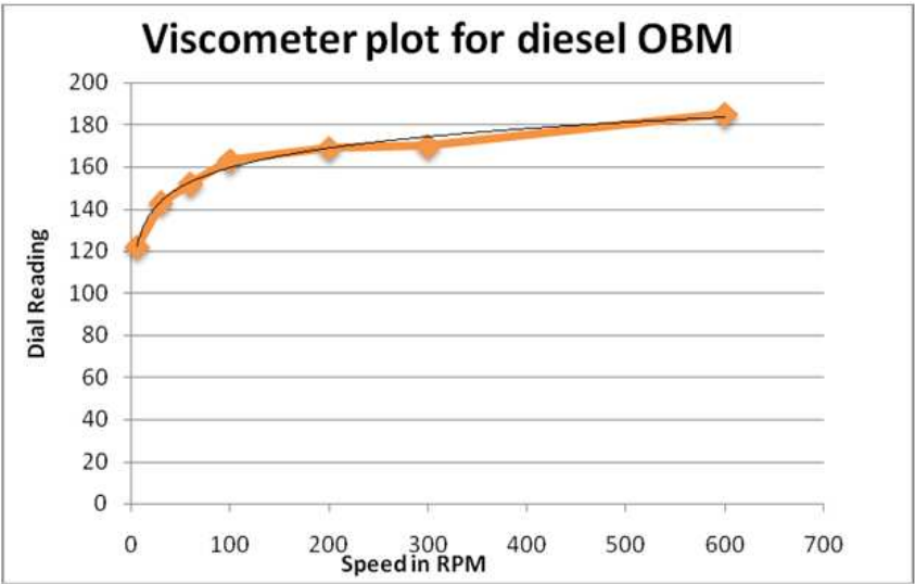
Figure 6. Viscometer Plot for Diesel OBM
