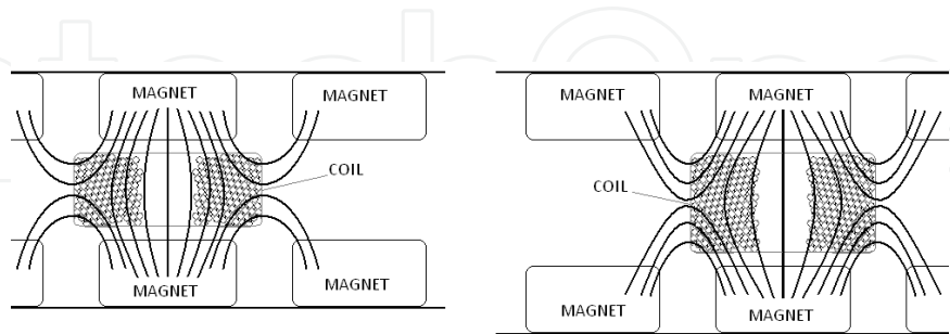
Figure 7. Lateral flux short circuiting to adjacent magnets increases (right) with increased rotor separation distance.
