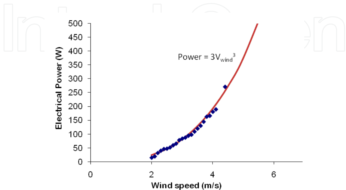
Figure 13. Electrical power versus wind speed at 9 degree attack angle with 6 ohm load
