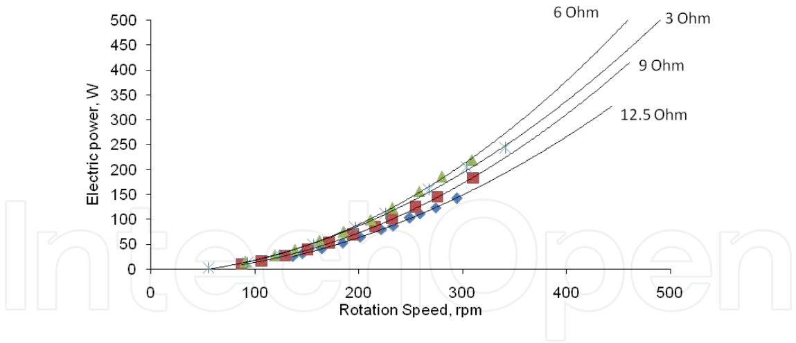
Figure 9. Power versus rotational speed for various loads
