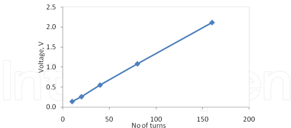
Figure 6. Individual coil open circuit voltage vs. number of turns at 50 rpm
