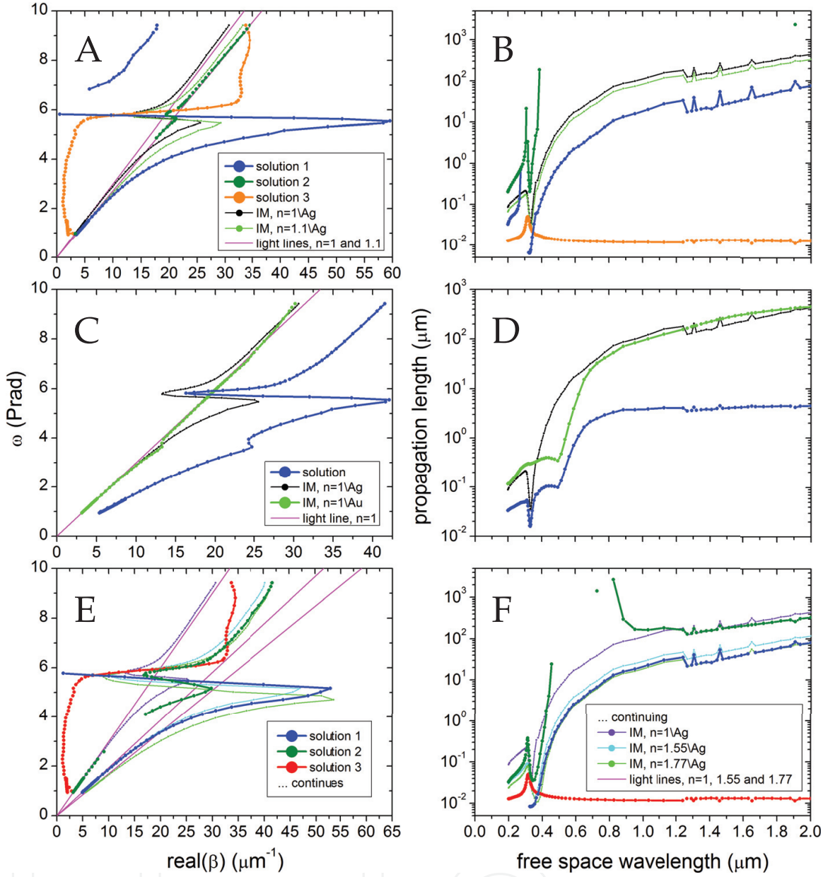
Figure 7. Dispersion relations and propagation lengths for asymmetric geometries modelling the metals by the tabulated permittivities. A, B) IMI: 25 nm silver layer surrounded by free space and other dielectric with n=1.1 . C, D) MIM: 25 nm free-space layer surrounded by silver and gold. E, F) IIMI: free space, 15 nm layer of a dielectric with n=1.77 , 45 nm silver layer and a dielectric with n=1.55 .
