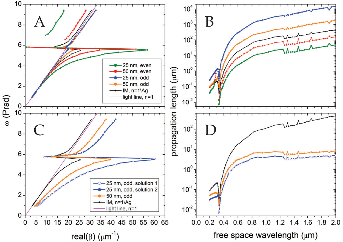
Figure 6. Dispersion curves and propagation lengths for symmetric geometries modelling the metals by the tabulated permittivities. A, B) IMI: 25 and 50 nm silver layer immersed in free space. C, D) MIM: 25 and 50 nm free-space layer immersed in silver.
