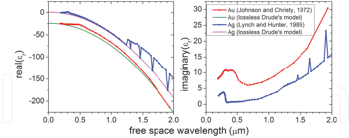
Figure 1. Permittivities of metals. Silver is modelled by the Drude's model without damping ( \omega_p = 13.1 Prad, \lambda_p = 144 nm) and the tabulated values of Lynch and Hunter (1985) [20]. Gold is modelled by the Drude's model without damping ( \omega_p = 13.4 Prad, \lambda_p = 141 nm) and the tabulated values of Johnson and Christy (1972) [13]. For easiness of visualisation, the real part of gold permittivity was shifted -25 units, and the imaginary part, +5 units.
