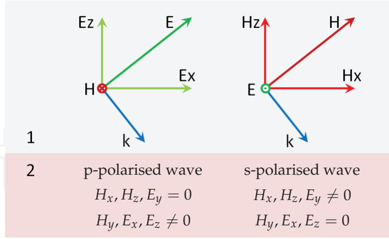
Figure 2. Interface between two media (1 and 2), showing the polarisation vectors of a p-polarised (left) and an s-polarised waves (right). The plane of incidence coincides with the page. A p-polarised wave (TM) is characterised by the magnetic field perpendicular to the plane of incidence; while an s-polarised (TE) wave is characterised by the electric field perpendicular to the plane of incidence.
