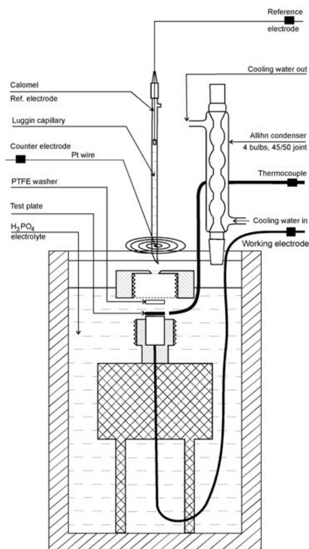
Figure 4. The electrochemical cell for corrosion testing in concentrated phosphoric acid.
