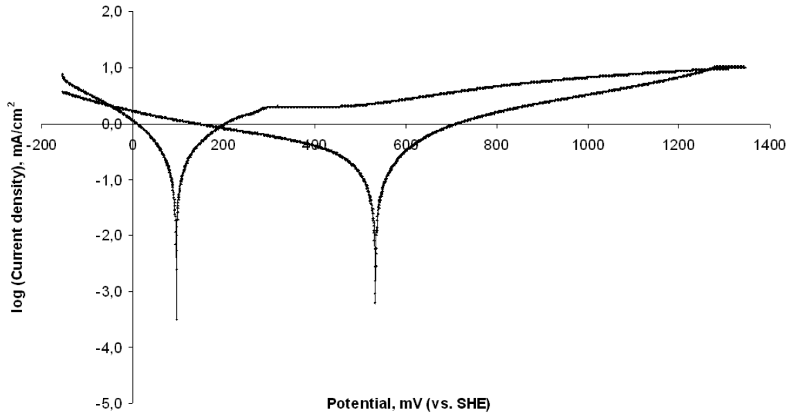
Figure 8. Tafel plot for AISI 316L in 85% H 3 PO 4 , 80 °C, 1 mV/s (vs. SHE).
