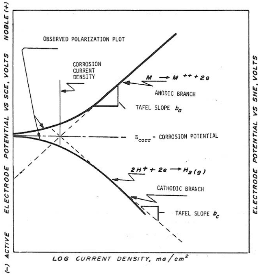
Figure 3. Hypothetical cathodic and anodic polarization diagram [3].
