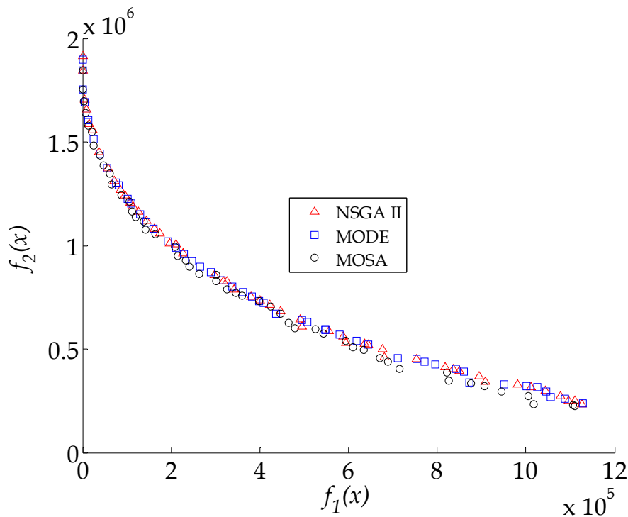
Figure 4. Pareto’s Front.
