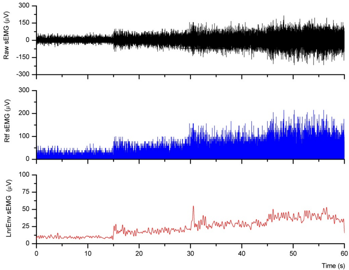
Figure 3. The raw sEMG (Raw sEMG), retificated (Rtf sEMG) and Linear envelope (LnrEnv sEMG) during ramp isometric contraction. Example figure.
