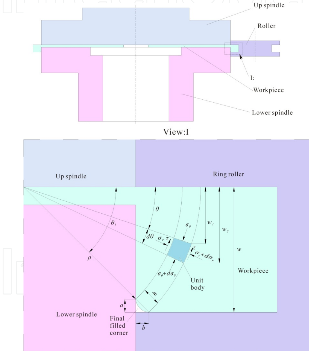
Figure 25. Sketch of principal stress on sector unit body
