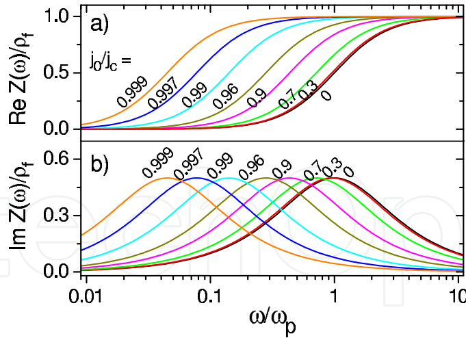
Figure 3. The frequency dependences of a) real and b) imaginary parts of the ac impedance calculated for a cosine pinning potential U_p(x) = (U_p/2)(1 - \cos kx) at a series of dc current densities, as indicated. In the absence of a dc current, the GR results are revealed in accordance with Eqs. (9).
