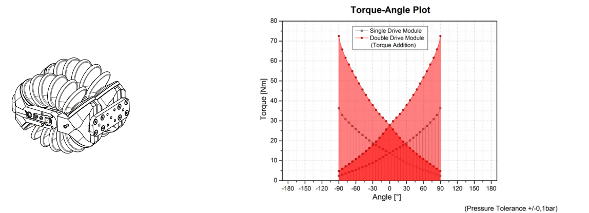
Figure 33. Double Module - Parallel Configuration
