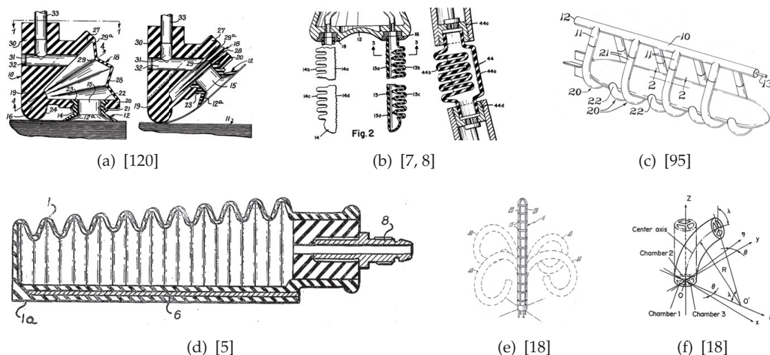
Figure 5. Bending Actuators
