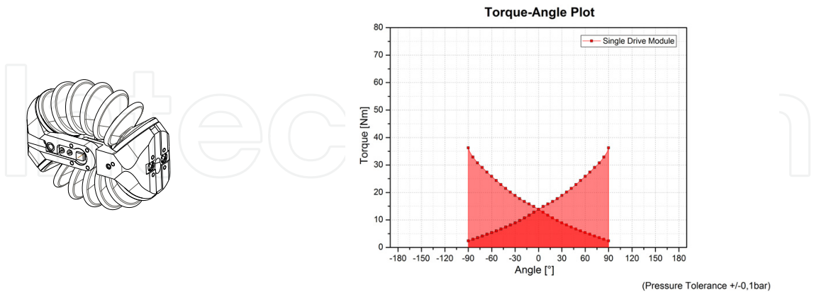
Figure 32. Single Drive Module
