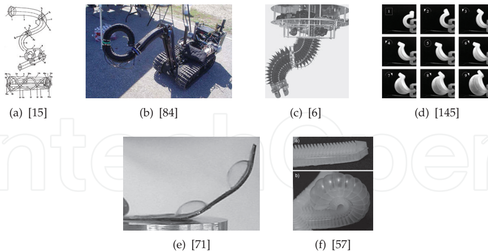
Figure 6. Trunk-Like Bending Actuators and Monolithic Bending Actuators
