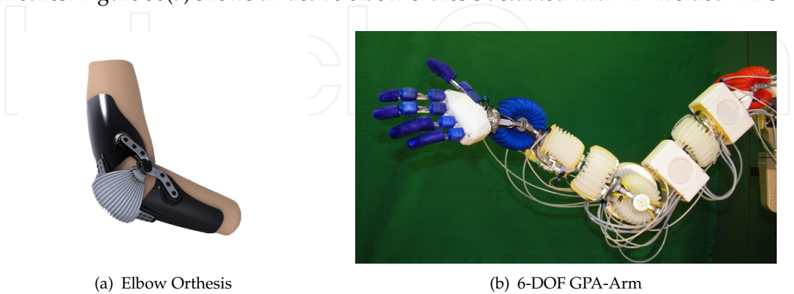
Figure 38. Systems with HF-welded Actuators
