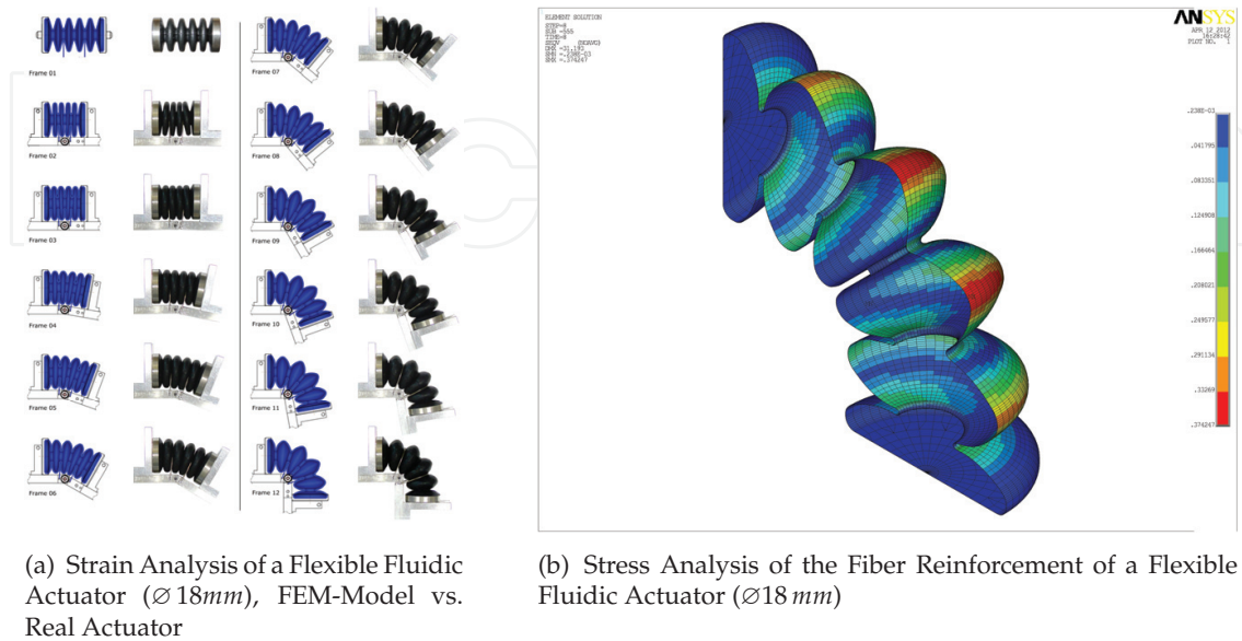
Figure 21. Structural Analysis of the Actuator Model
