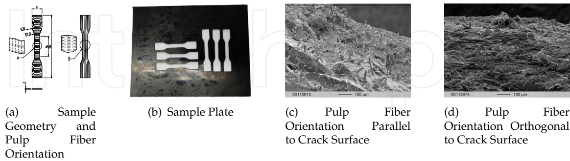
Figure 13. Material Characterization
