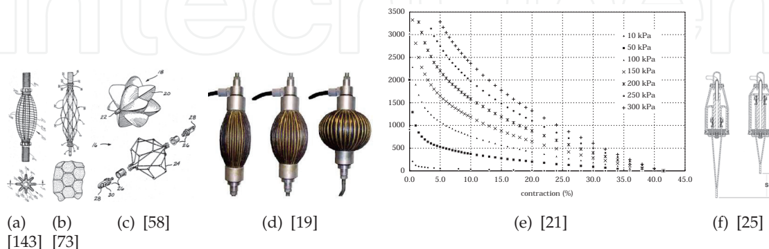
Figure 4. Some FFAs based on “Vectored Structural Degrees of Freedom”
