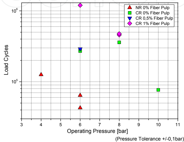
Figure 16. Fatigue Resistance of 18 mm -Actuators
