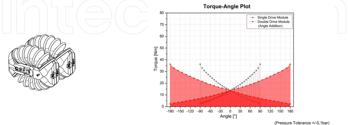
Figure 34. Double Module - Serial Configuration
