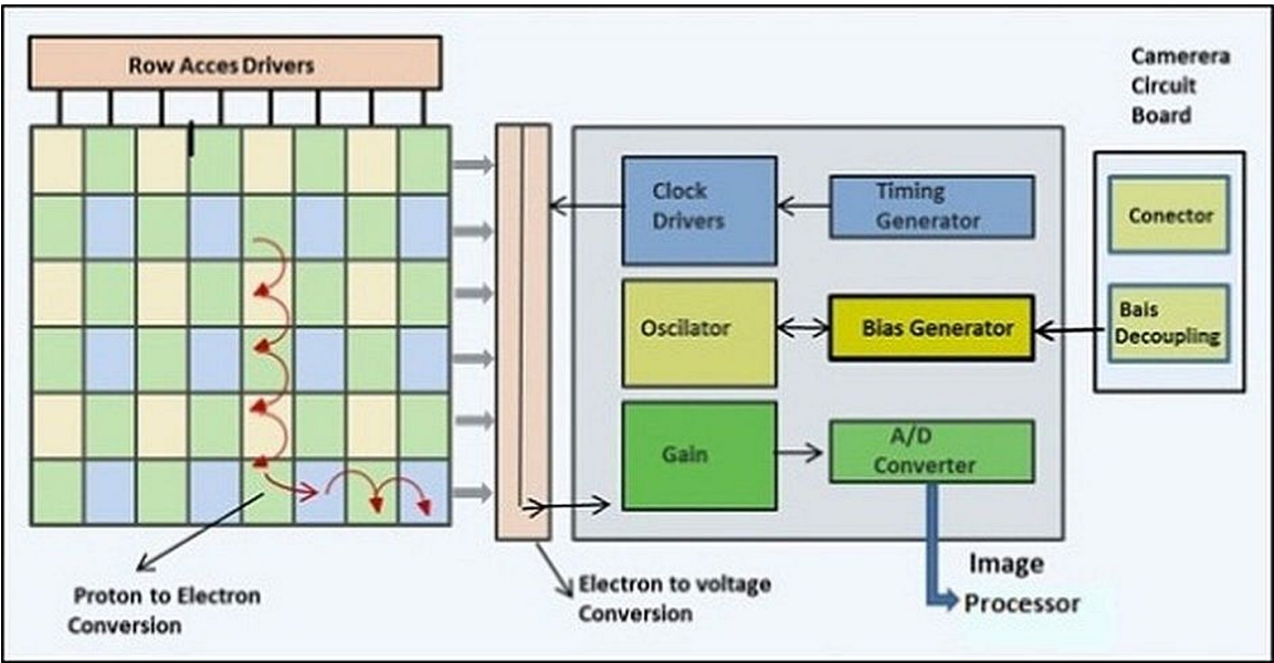
Figure 14. CMOS sensor.
