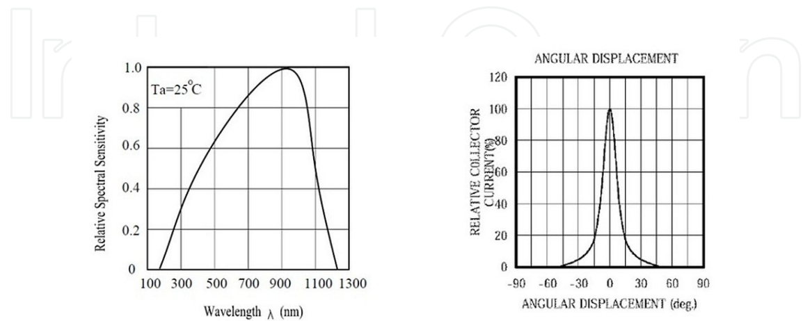
Figure 11. Relative spectral sensitivity and collector current vs. angular displacement of a phototransistor.
