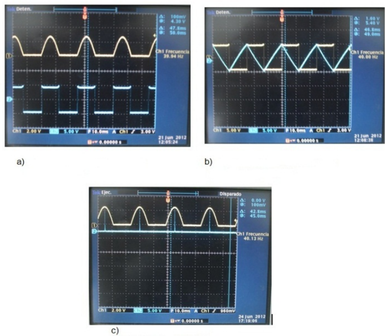
Figure 27. Detailed example. a)Channel 1: original signal from function generator; Channel 2: square signal obtained from saturation. b) Channel 1: saturated signal Channel 2: ramp signal obtained from integration. c) Channel1: original signal from generator; Channel 2: impulse signal overlapped on original signal from generator to indicate the energetic signal centre.
