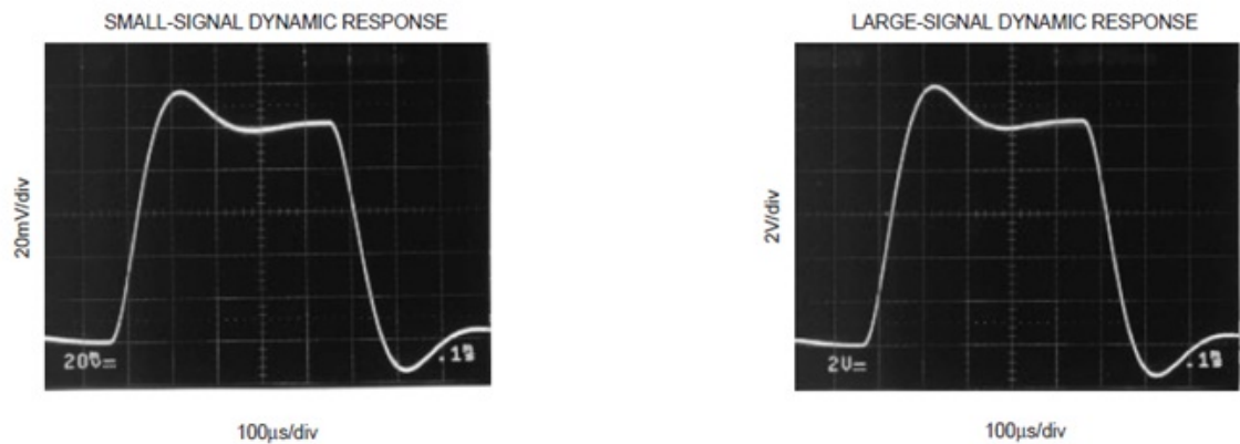
Figure 10. Small and large signal dynamic response of a photodiode.
