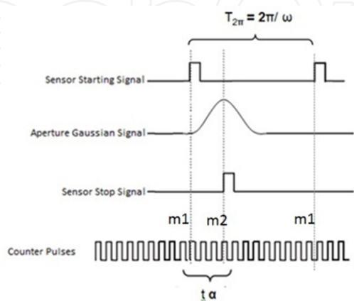
Figure 7. Signal generated by a 45° cylindrical mirror scanner.
