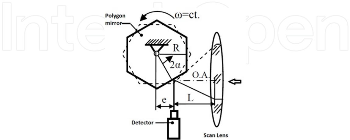
Figure 3. Polygon scanner.
