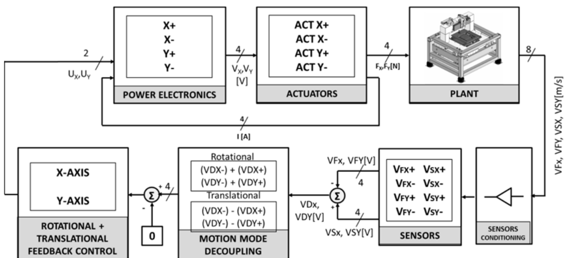
Figure 24. Modal control overall scheme.
