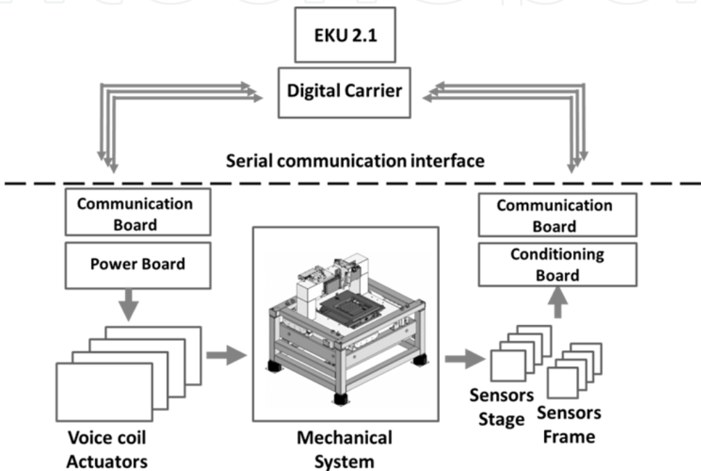
Figure 10. Electronics subsystem.
