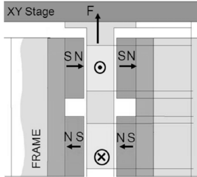
Figure 5. Actuator force generation.
