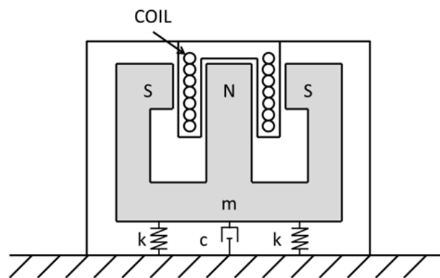
Figure 8. Geophone reverse configuration scheme.
