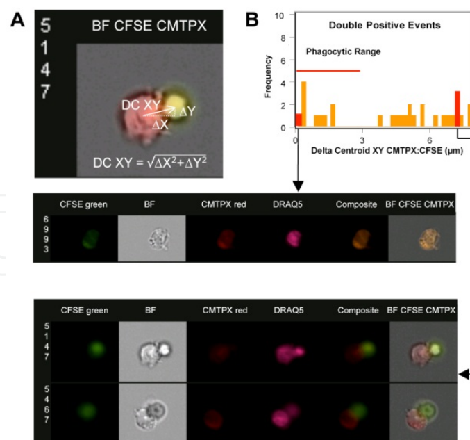
Figure 5. Delta centroid image analysis to identify phagocytosis in double positive events. Panel A shows a composite image of brightfield, CFSE, and CMTPIX fluorescence in a double positive event of U-937 effector cells and Ramos target cells incubated for 2 h in the presence of 5 \mu\text{g/ml} rituximab. Superimposed is the vector used to calculate the distance between the centers of the masks of the
