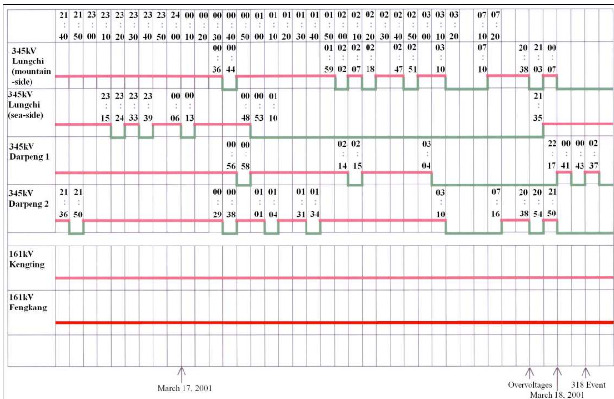
Figure 2. 345kV and 161kV Overhead Line Switching Event Log
