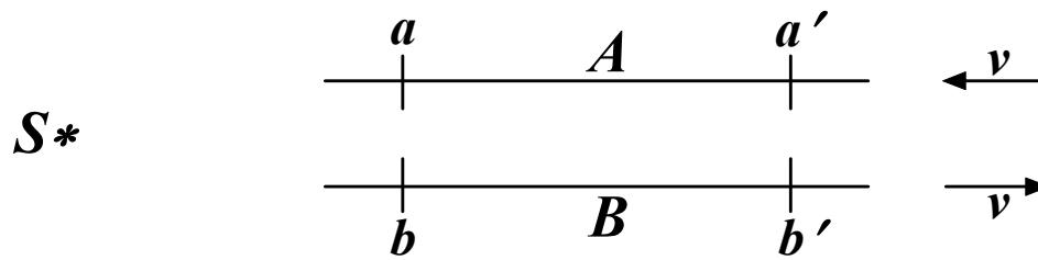
Figure 4. Test of Light Speed Invariance
