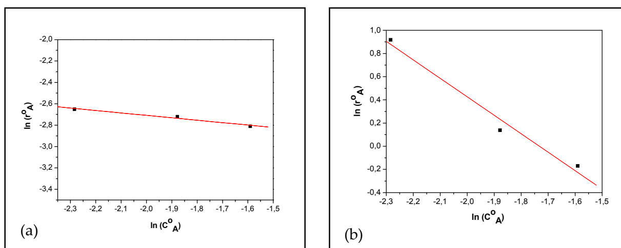
Figure 10. Initial reaction rate of 1-heptyne concentration for (a) Ni/Al 2 O 3 and (b) Pd/Al 2 O 3 . P_{H_2}=1.4 bar, T=303 K, 800 rpm, W_{\text{cat}}=0.3 g Ni/Al 2 O 3 or 0.03 g Pd/Al 2 O 3 , S/\text{Ni}=42, 64 and 85 , S/\text{Pd}=19596, 29335 and 39192 .
