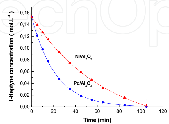
Figure 4. C_A vs. reaction time. P_{\text{H}_2} = 1.4\ \text{bar} , C_A^0 = 0.1528\ \text{mol L}^{-1} , T = 323\ \text{K} , 800 rpm, W_{\text{cat}} = 0.3\ \text{g}_{\text{Ni}/\text{Al}_2\text{O}_3} or 0.03\ \text{g}_{\text{Pd}/\text{Al}_2\text{O}_3} , S/\text{Ni} = 64 and S/\text{Pd} = 29385 .
