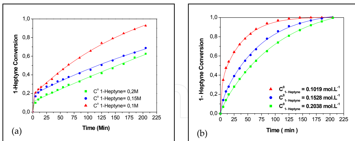
Figure 9. Effect of C_A^0 on the catalytic activity for (a) Ni/Al 2 O 3 and (b) Pd/Al 2 O 3 . P_{H_2}=1.4 bar, T=303 K, 800 rpm, W_{\text{cat}}=0.3 g Ni/Al 2 O 3 or 0.03 g Pd/Al 2 O 3 , S/\text{Ni}=42, 64 and 85 , S/\text{Pd}=19596, 29335 and 39192 .
