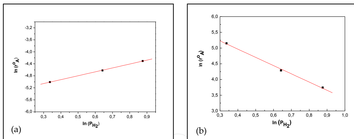
Figure 8. Initial reaction rate as a function of hydrogen pressure for (a) Ni/Al 2 O 3 and (b) Pd/Al 2 O 3 . C_A^0 = 0.1528 \text{ mol L}^{-1} , T = 303 \text{ K} , 800 rpm, W_{\text{cat}} = 0.3 \text{ g}_{\text{Ni/Al}_2\text{O}_3} or 0.03 \text{ g}_{\text{Pd/Al}_2\text{O}_3} , S/\text{Ni} = 64 and S/\text{Pd} = 29385 .
