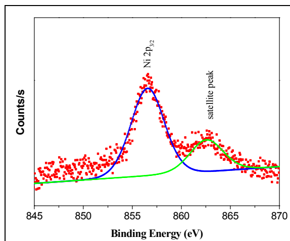
Figure 1. XPS Ni 2p 3/2 spectra of Ni/Al 2 O 3 .
