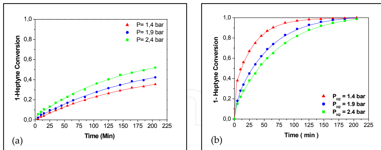
Figure 7. Effect of P_{H_2} on the catalytic activity for (a) Ni/Al 2 O 3 and (b) Pd/Al 2 O 3 . C_A^0 = 0.1528 \text{ mol L}^{-1} , T = 303 \text{ K} , 800 rpm, W_{\text{cat}} = 0.3 \text{ g}_{\text{Ni/Al}_2\text{O}_3} or 0.03 \text{ g}_{\text{Pd/Al}_2\text{O}_3} , S/\text{Ni} = 64 and S/\text{Pd} = 29385 .
