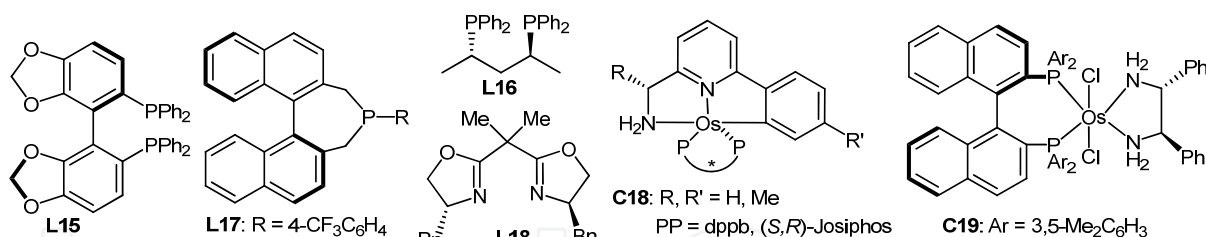
Figure 10. Ligands for Cu-mediated hydrogenation and Os-complexes
