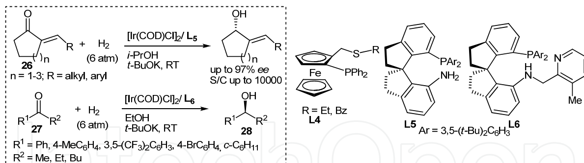
Figure 6. Ir-catalyzed AH
