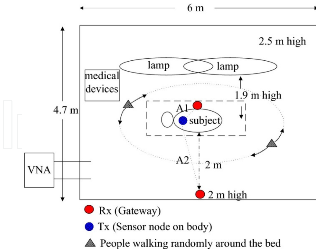
Figure 2. Floor plan of a regular hospital room.
