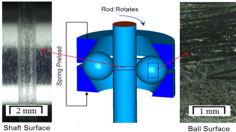
Figure 8. Autopsy data for RCF elements in configuration 1 of Table 1 operated at 3.61 GPa loading. Suspension after 1.7 hours of rotation at 130 Hz, accounting for approximately 7.8 \times 10^5 rod stress cycles.
