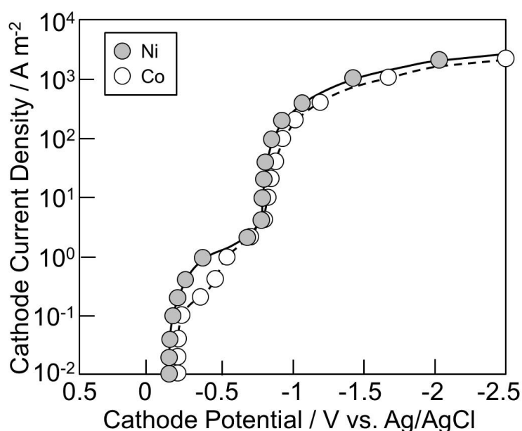
Figure 10. Cathode polarization curves for Ni and Co electrodeposition from aqueous solution containing \text{Ni}^{2+} or \text{Co}^{2+} ions.
