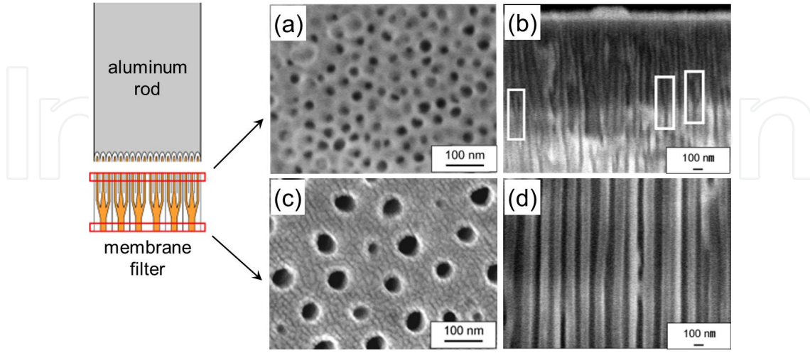
Figure 6. SEM images of barrier layer side (plan view (a), cross section (b)) and surface side (plan view (c), cross section (d)) of an anodized aluminum oxide membrane filter exfoliated from a metallic aluminum rod. The anodization was conducted at 70 V.
