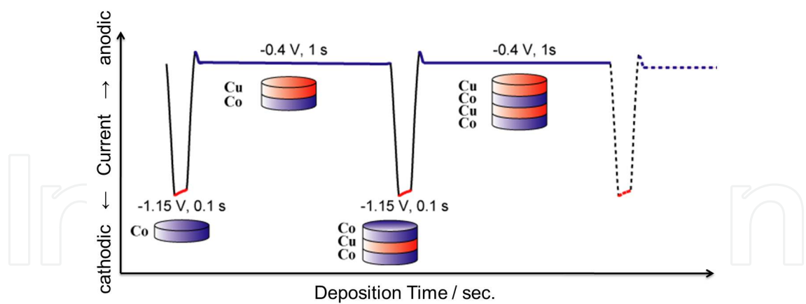
Figure 18. Growing process of Co/Cu multilayered nanowires synthesized alternately switching cathode potential from -0.4 V (for Cu layer) to -1.15 V (for Co layer).
