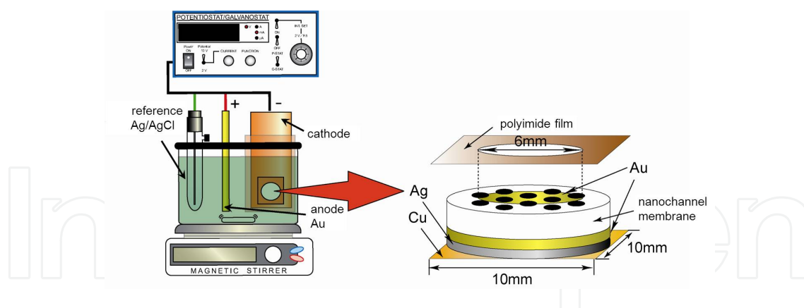
Figure 9. Experimental apparatus and a nanochannel template for electrodeposition of nanowires array.
