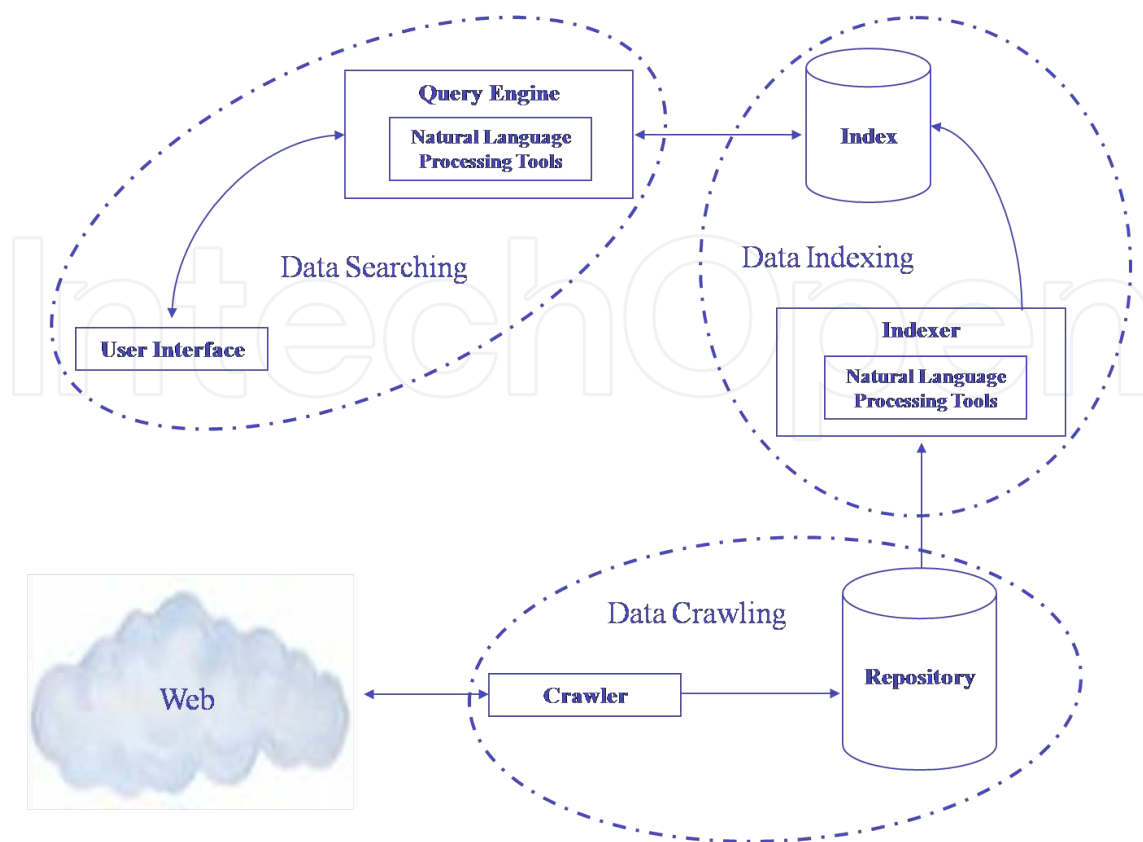
Figure 4. Amazigh search engine architecture.
