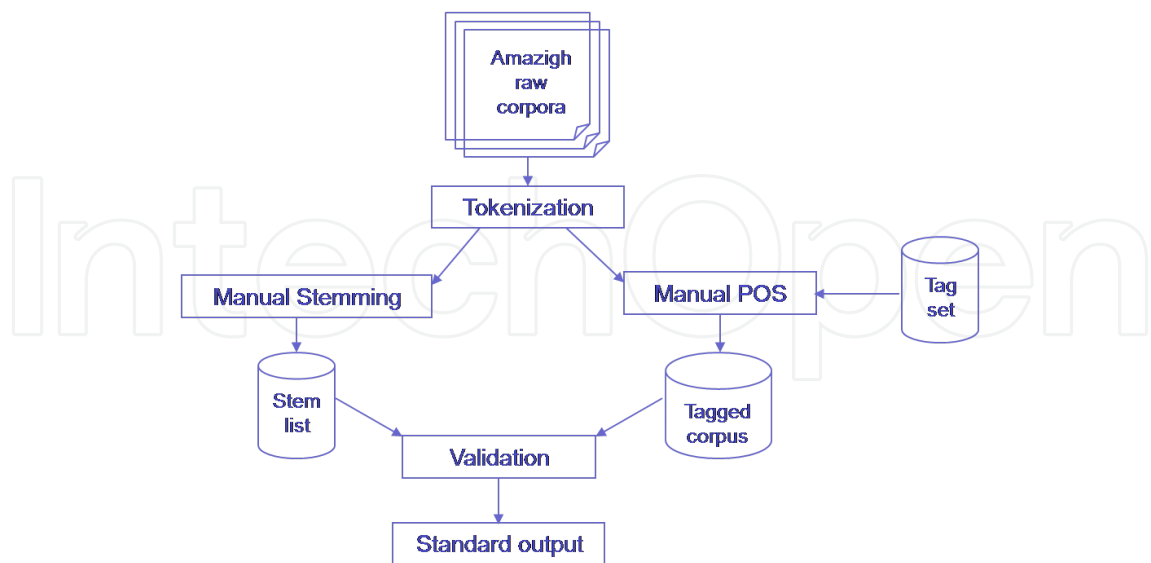
Figure 6. Tagging assistance tool conception.
