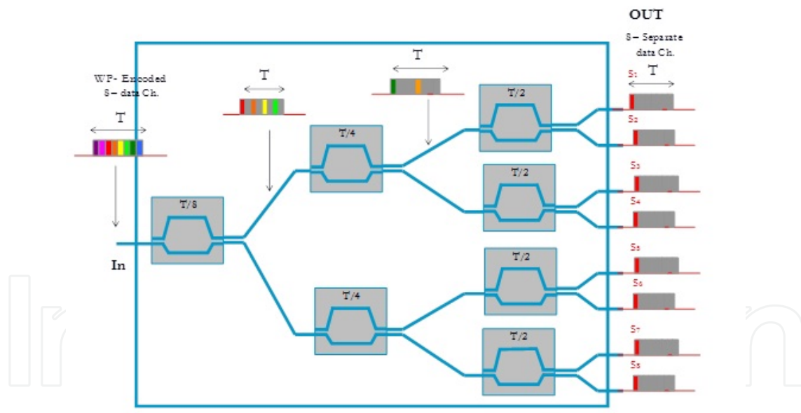
Figure 8. All-optical Haar WP Decoder used as an optical receiver
