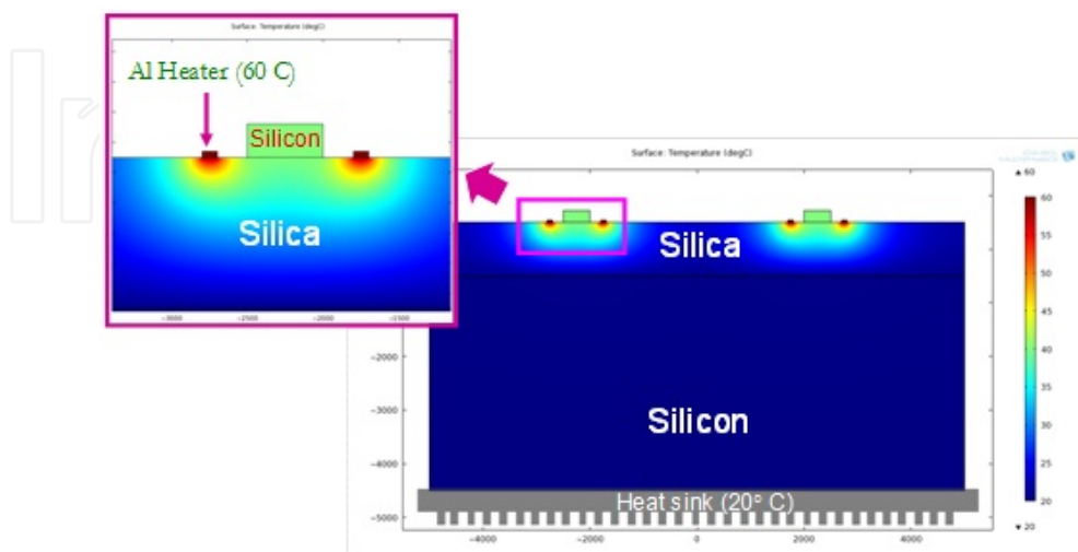
Figure 12. Cross section of heat dissipation in an SOI waveguide with the aluminium heaters located in both sides of the SOI waveguide
