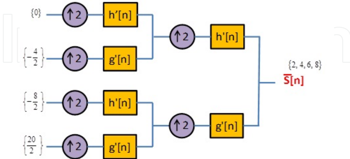
Figure 4. Haar inverse wavelet-packet decomposition (IWPDP) transform
