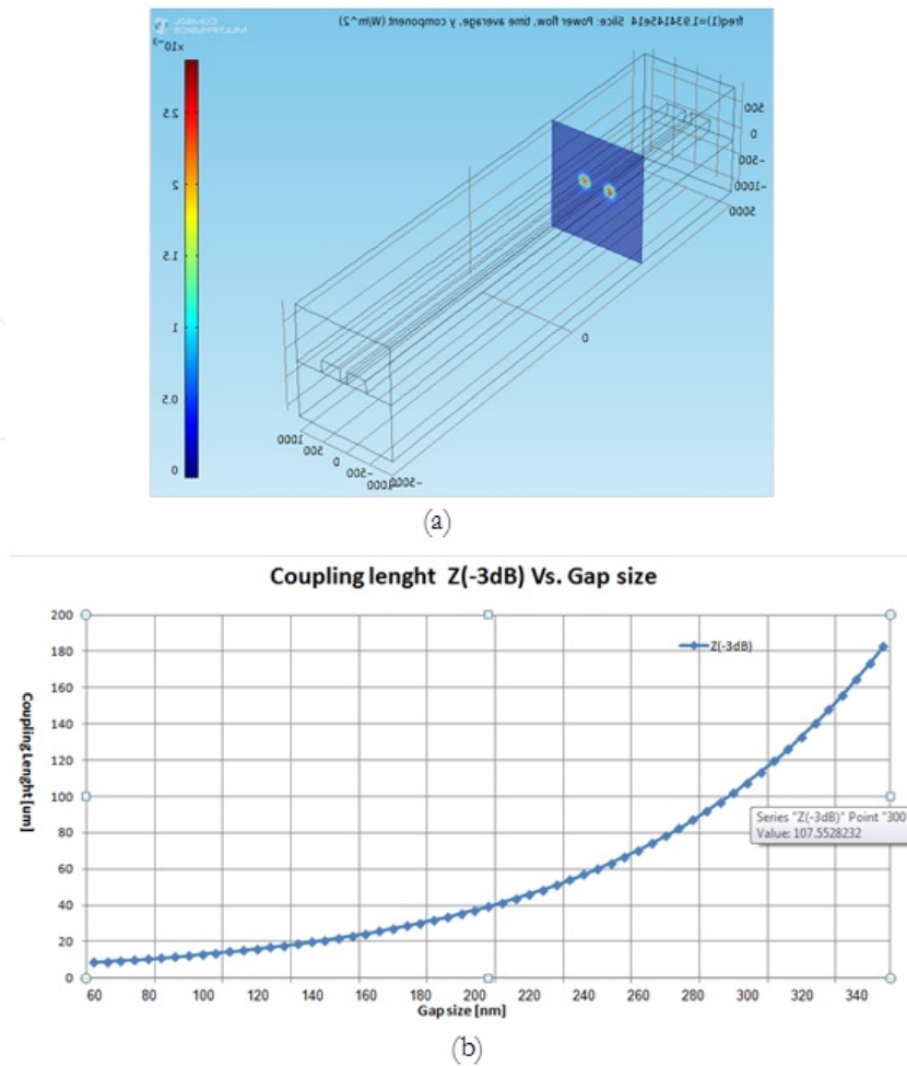
Figure 11. Coupler dimensions design with COMSOL software simulations: (a) an example of a three-dimensional modelling of a directional coupler; (b) calculated coupling length that is required between two parallel waveguides as a function of the gap size. The coupling length for the chosen gap size of 300 nm is approximately 110\mu\text{m}
