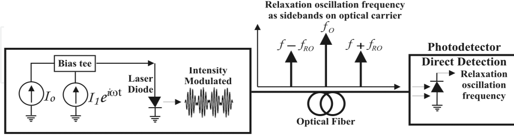
Figure 8. Direct detection to generate relaxation oscillation frequency when laser is operated in low threshold region.
