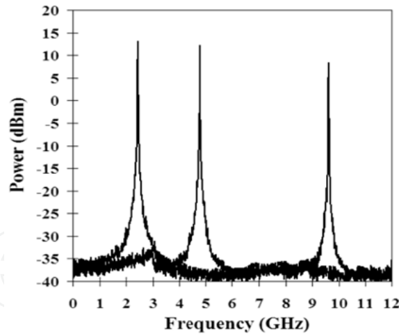
Figure 3. Microwave spectrums continuously tuned from 0 to 10 GHz.
