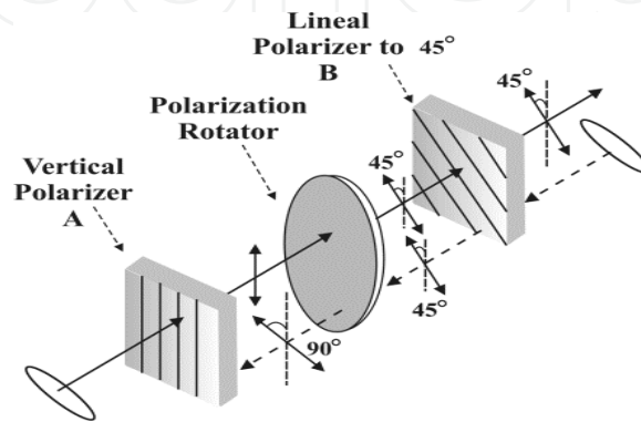
Figure 15. Principle of operation of an optical isolator.
