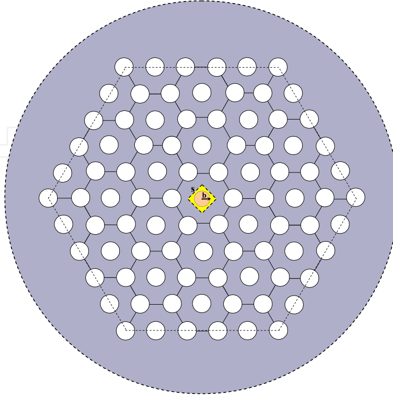
Figure 5. Transverse structure of the MHOF (The air holes in the fifth layer from the core are linked by the dashed line, forming a hexagonal ring.)
