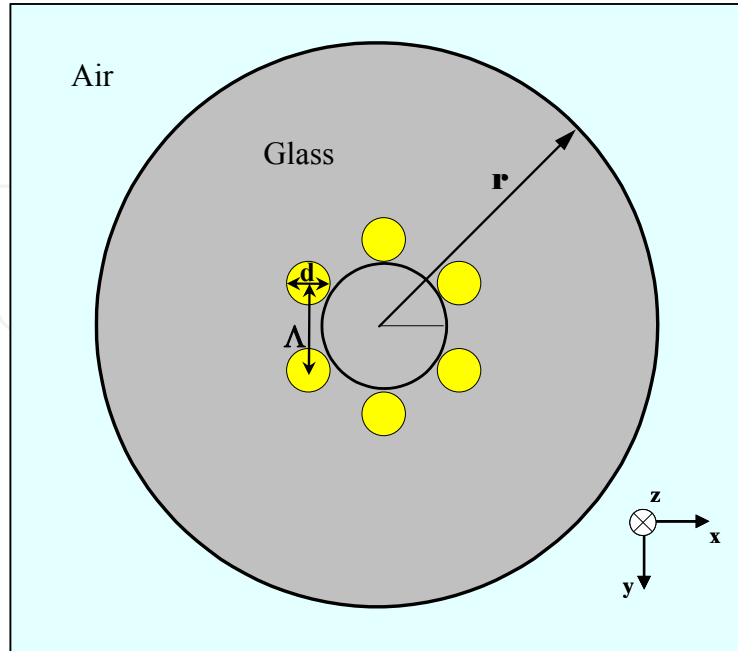
Figure 3. Schematic of a cross section for an MHOF with one layer of air holes in a hexagonal arrangement
