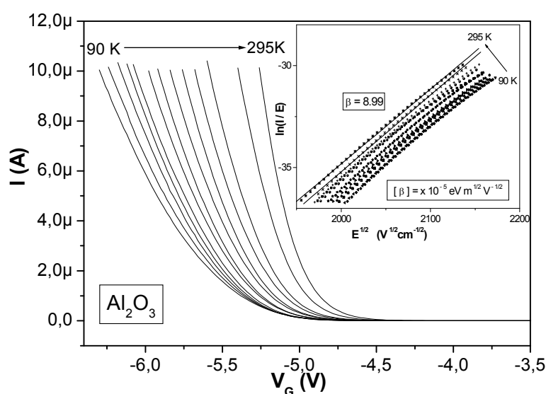
Figure 4. I-V curves at several temperatures and Poole-Frenkel fitting of an ALD \text{Al}_2\text{O}_3 -based MIS sample
