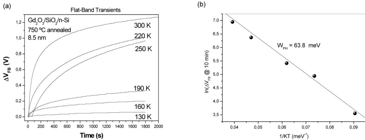
Figure 25. Flat-band voltage transients at different temperatures (a) and Arrhenius plot of the transient amplitude at 10 minutes (b) for an \text{Al}/\text{Gd}_2\text{O}_3/\text{SiO}_2/\text{Si} sample.
