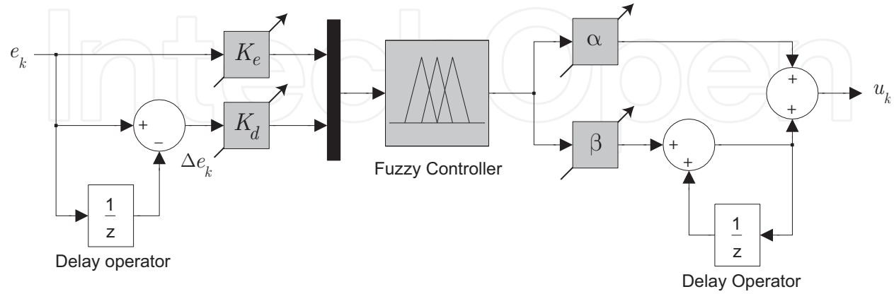
Figure 1. The proposed discrete-time PID-type FC structure.
