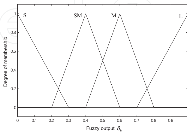
Figure 4. Membership functions for \delta_k .
