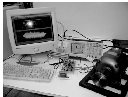
Figure 15. The developed experimental DC drive benchmark.
