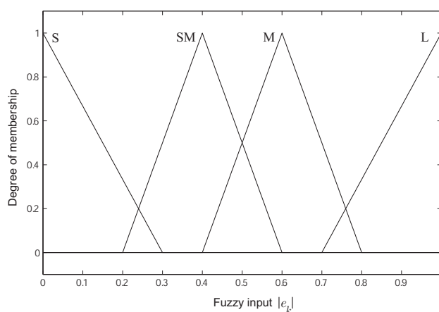
Figure 3. Membership functions for |e_k| .
