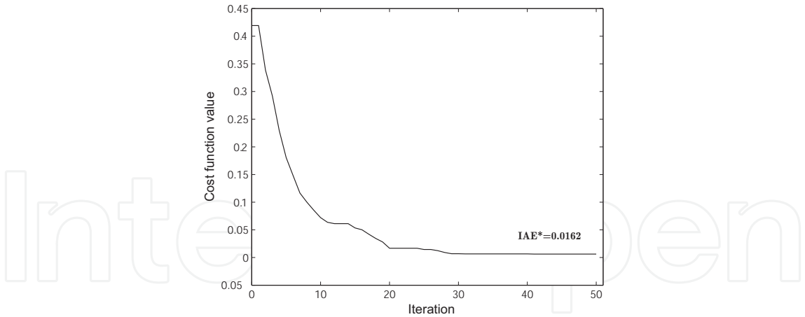
Figure 8. Convergence properties of the proposed PSO algorithm: IAE criterion case.
