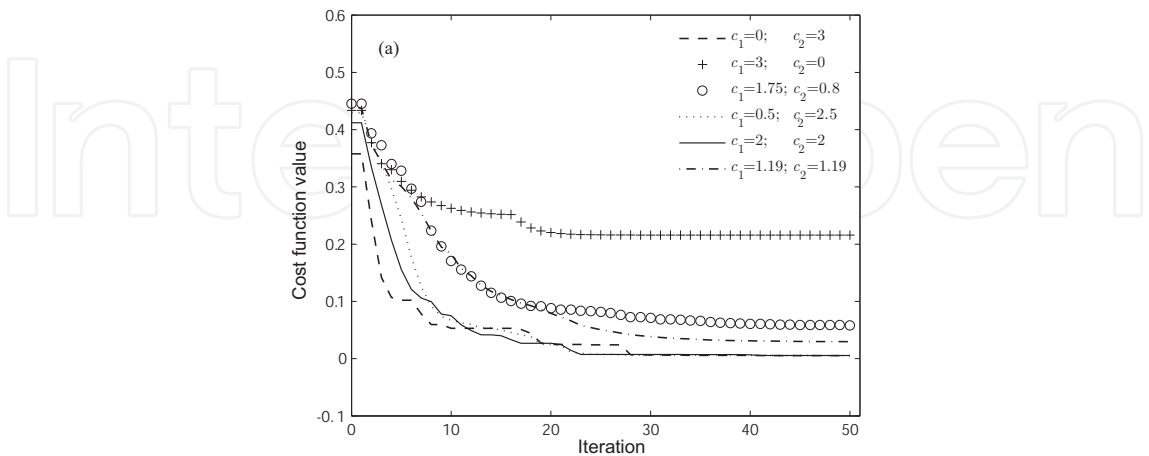
Figure 10. Robustness of the proposed PSO algorithm under variations of the cognitive and social parameters: IAE criterion case.
