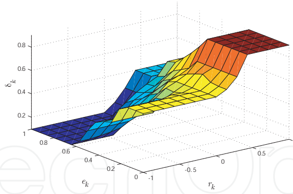
Figure 5. View of the fuzzy rule-base for \delta_k .
