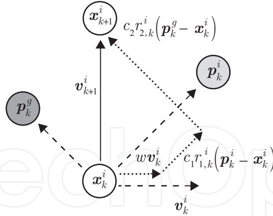
Figure 6. Particle position and velocity updates.
