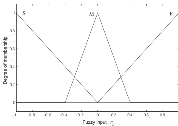
Figure 2. Membership functions for r_k .
