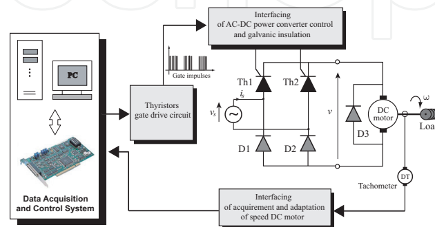
Figure 14. The proposed experimental setup schematic.
