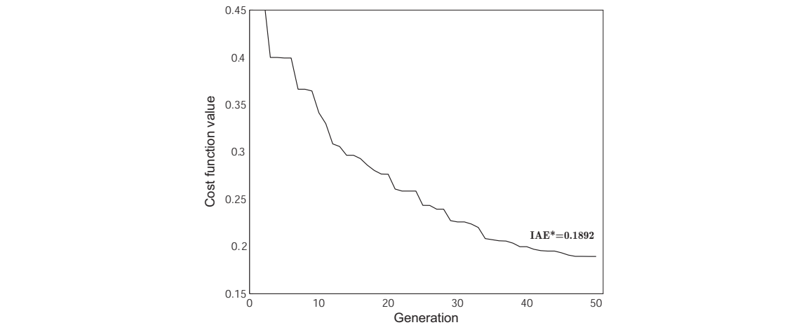
Figure 9. Convergence properties of the standard GAO algorithm: IAE criterion case.
