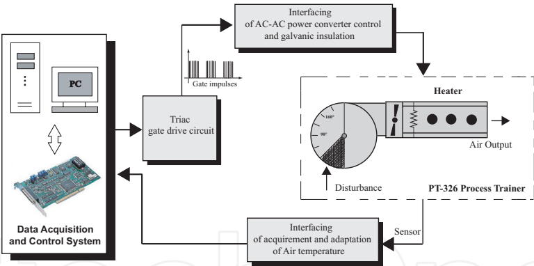
Figure 19. The proposed thermal process experimental setup schematic.
