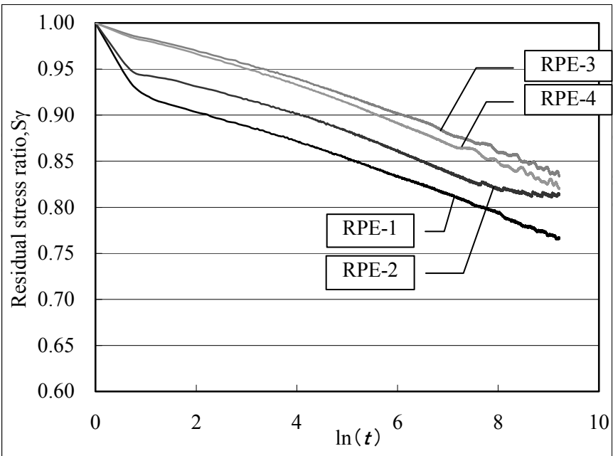
Figure 11. Compression relaxation curve (RPE-1,2,3,4, disp.=5cm)
