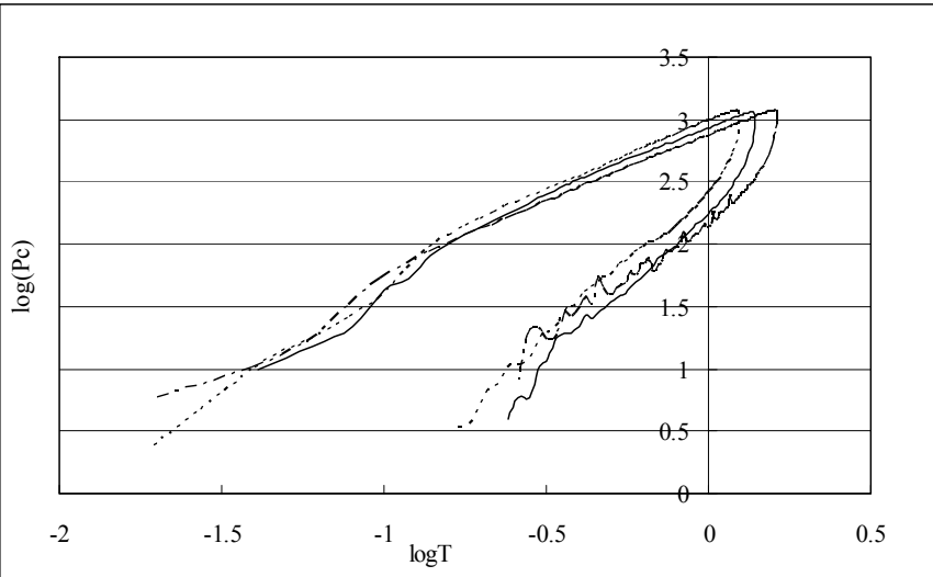
Figure 9. A plot of the relationship between the logarithm of compression stress and the logarithm of thickness change at 6th cycle. Straight line: WPE-1 Dotted line: RPE-1 Dots and dashes: CU-1
