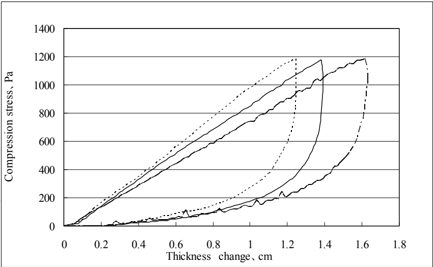
Figure 8. Compression-recovery curve at 6th cycle under the condition that volume fraction is 0.0125 and maximum compression stress is 1176 Pa for three samples. Straight line: WPE-1 Dotted line: RPE-1 Dots and dashes: CU-1
