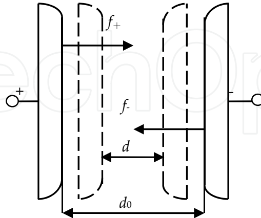
Figure 2. Electromechanical breakdown model
