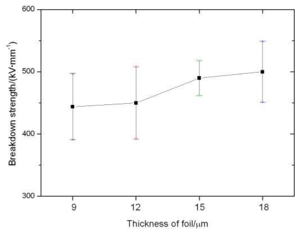
Figure 10. Breakdown strength for thickness-varied polyester-foil under negative voltage
