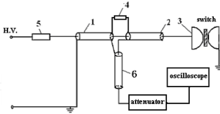
Figure 5. Electrical schematic diagram of experiment
