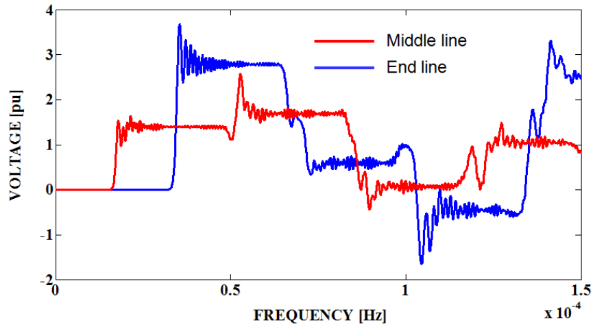
Figure 29. The time domain simulations with the corona effect for V_{\text{CORONA}} = 0,7 \text{ V} .
