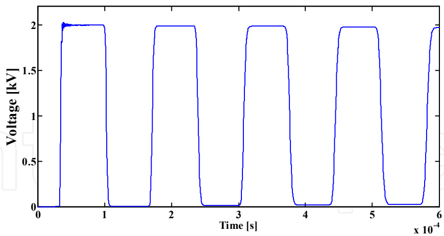
Figure 24. Voltage at the end of the line with the effect of frequency considering 200 \pi circuits and using R_4L_4 parallel block.
