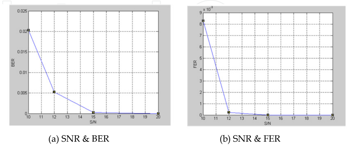
Figure 11. Relationship between SNR & (BER, FER)
