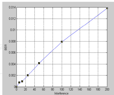
(a) Interference &amp; BER
