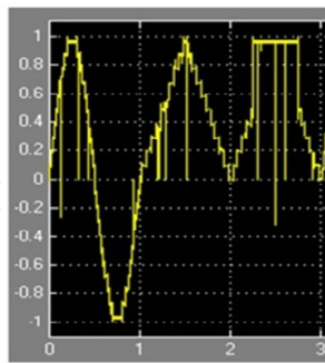
(a) SNR=15dB, Average Rate=6
