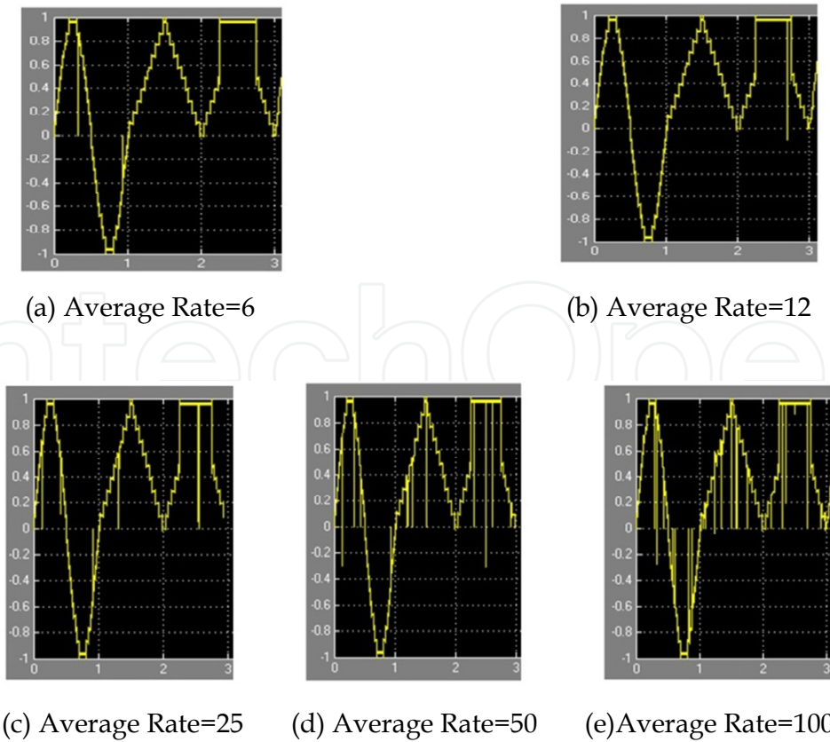
Figure 6. Received signals with different rate of interference
