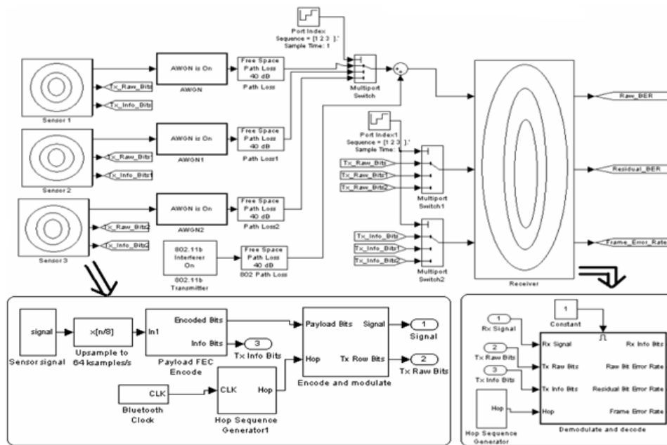
Figure 2. Simple WSN model
