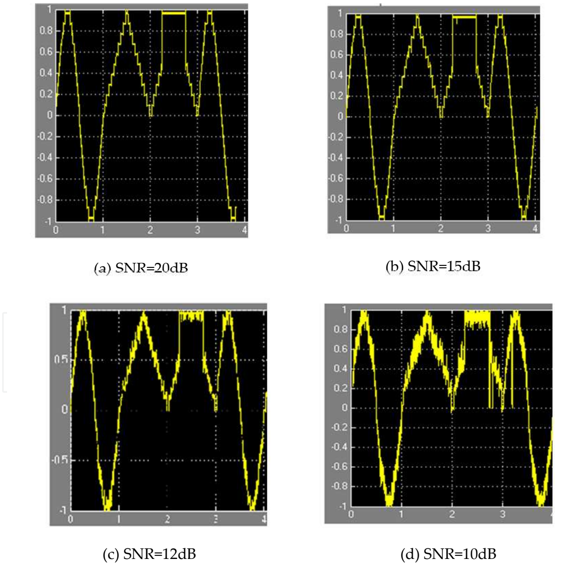
Figure 4. Received signals with different SNR
