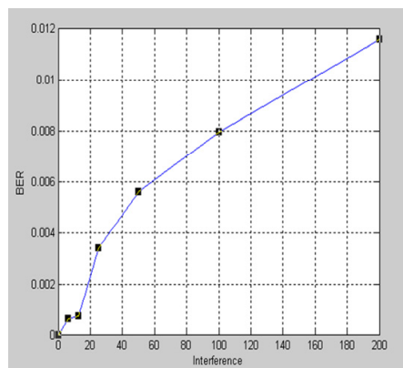
(a) Interference &amp; BER
