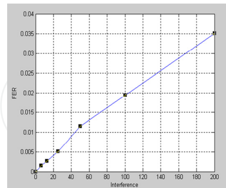
(b) Interference &amp; FER
