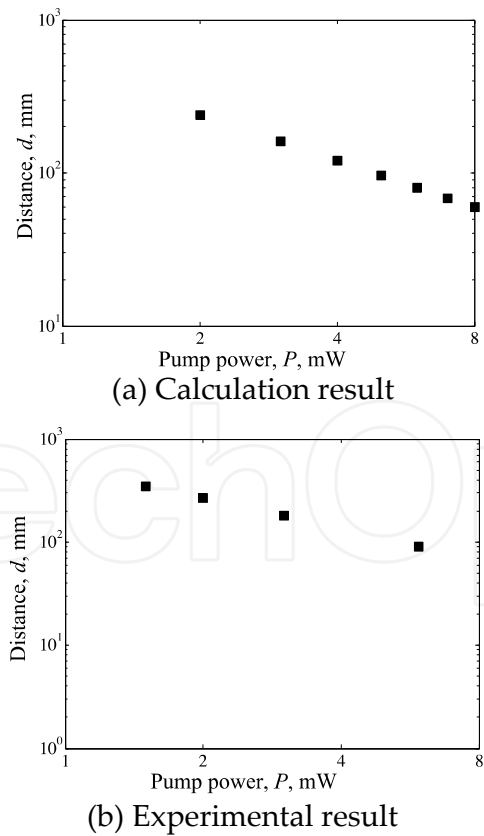
Figure 14. Relationship between the pump power and the distance to obtain the flat-top beam profile. The horizontal and vertical axes show the pump power and the distance to obtain the flat-top beam profile respectively.
