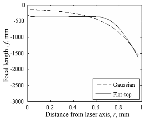
Figure 16. Effect of the pump beam profile to the focal length of the GRIN-L lens
