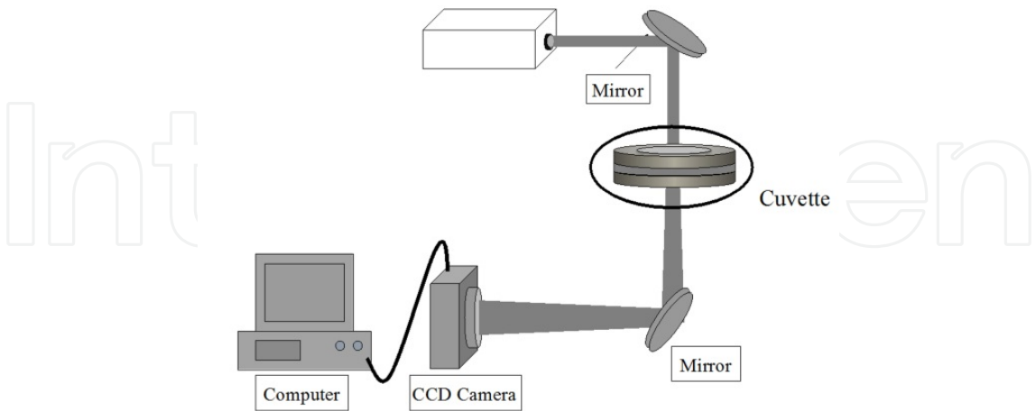
Figure 11. Experimental set up for a single-beam thermal lens system to transfer a Gaussian beam to flat-top beam
