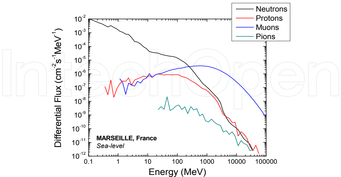
Figure 2. High energy ( > 0.1 \text{ MeV} ) differential flux for atmospheric neutrons, protons, muons and pions at ground level. Data computed using the QinetiC Atmospheric Radiation Model [22-23] for Marseille, France (Latitude 43.18^\circ \text{ N} , Longitude 5.22^\circ \text{ E} , sea-level).
