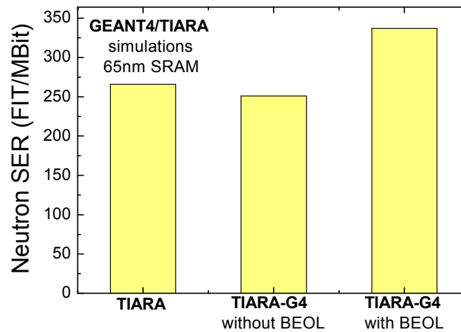
Figure 15. Comparison of simulation results obtained with the initial (TIARA) and new (TIARA-G4) versions of the code for the evaluation of the neutron-induced SER in the 65 nm SRAM architecture. Data are also plotted for TIARA-G4 with and without taking into account the real BEOL structure.
