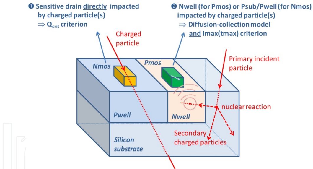
Figure 8. Schematics of the different cases envisaged in TIARA-G4 for the evaluation of cell upset in the simulated SRAM circuit.
