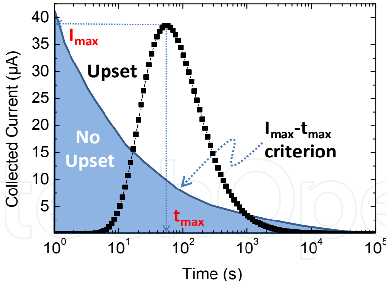
Figure 10. Example of a transient current characteristic superimposed to the I_{\max} - t_{\max} upset criterion. The transient current has been calculated from the “diffusion-collection model” for a ^{24}\text{Mg} particle (10 MeV) which perpendicularly impacts a Pwell at the distance of 0.25 \mu\text{m} from the Nmos drain contact.
