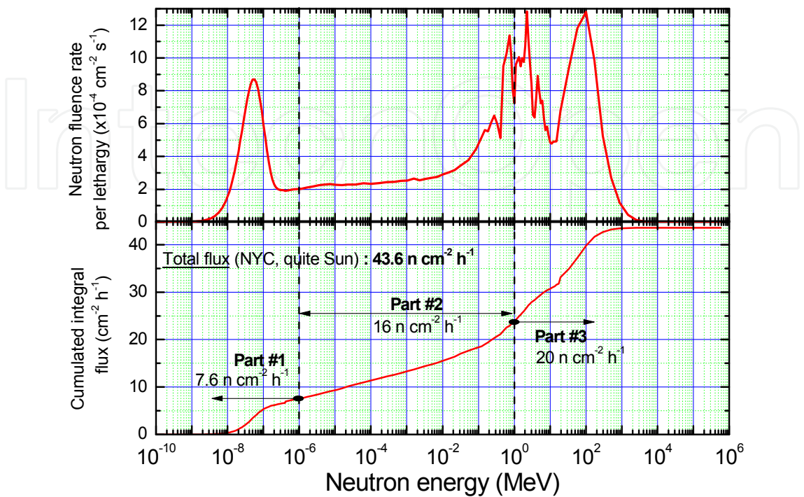
Figure 1. Top: Reference atmospheric neutron spectrum measured on the roof of the IBM Watson Research Center main building [21]. Numerical data courtesy from Paul Goldhagen (U.S. Department of Homeland Security). Bottom: Cumulated integral flux corresponding to the above spectrum. The total neutron flux is 43.6 neutrons per \text{cm}^2 and per hour.
