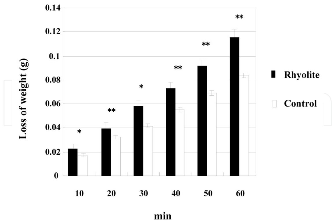
Figure 10. The change of the deionized water weight affected by the rhyolite as the FIR radiator
