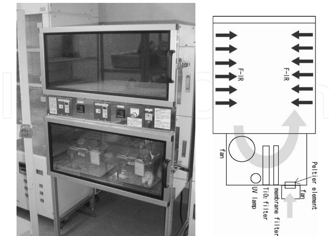
Figure 8. The FIR animal raising apparatus
