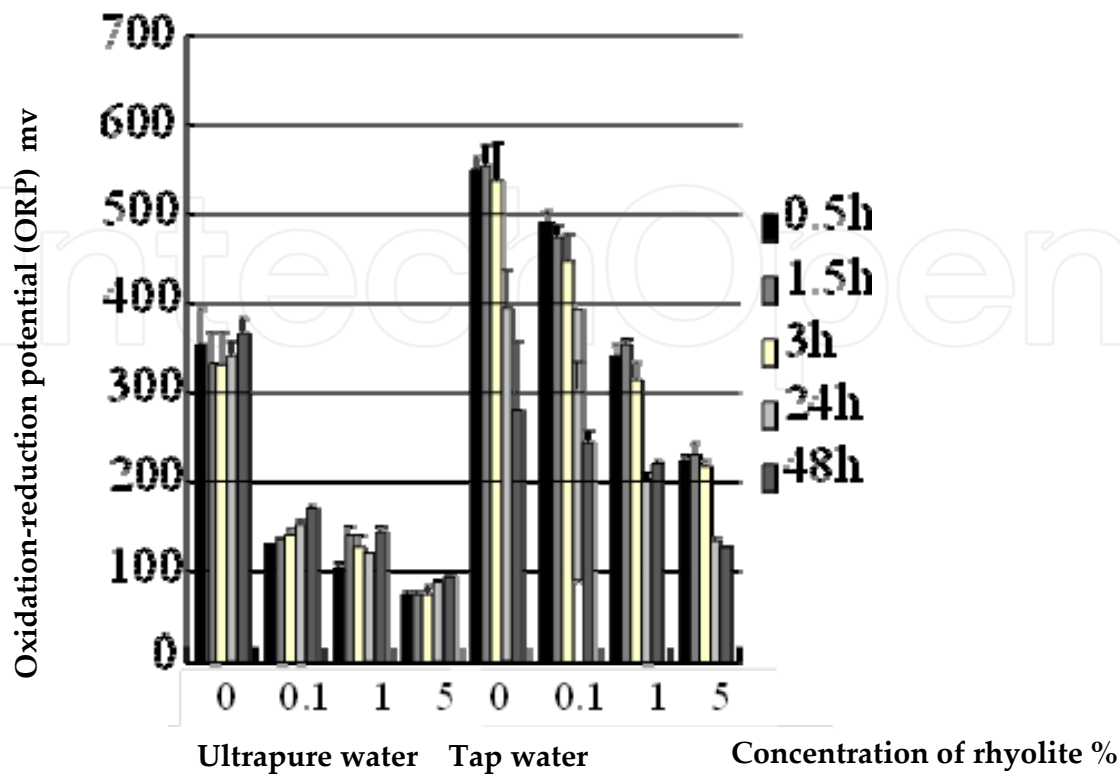
Figure 5. The change of the oxidation-reduction potential affected by the rhyolite. The oxidation-reduction potential (The longitudinal axis shows ORP, mv) decreased depending on the contents of the rhyolite(The transverse axis shows %) after 0.5-48h.
