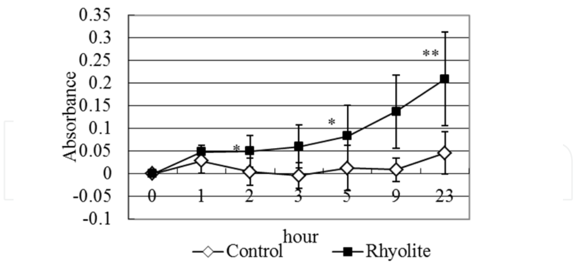
Figure 12. The solubility of BSA in the FIR energy radiated water
