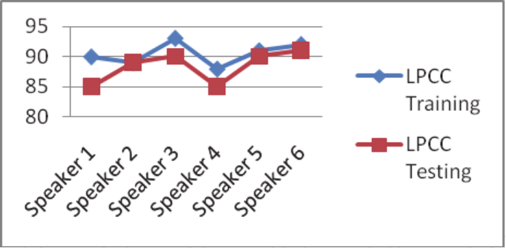
Figure 13. LPCC speaker identification rate with conventional system
