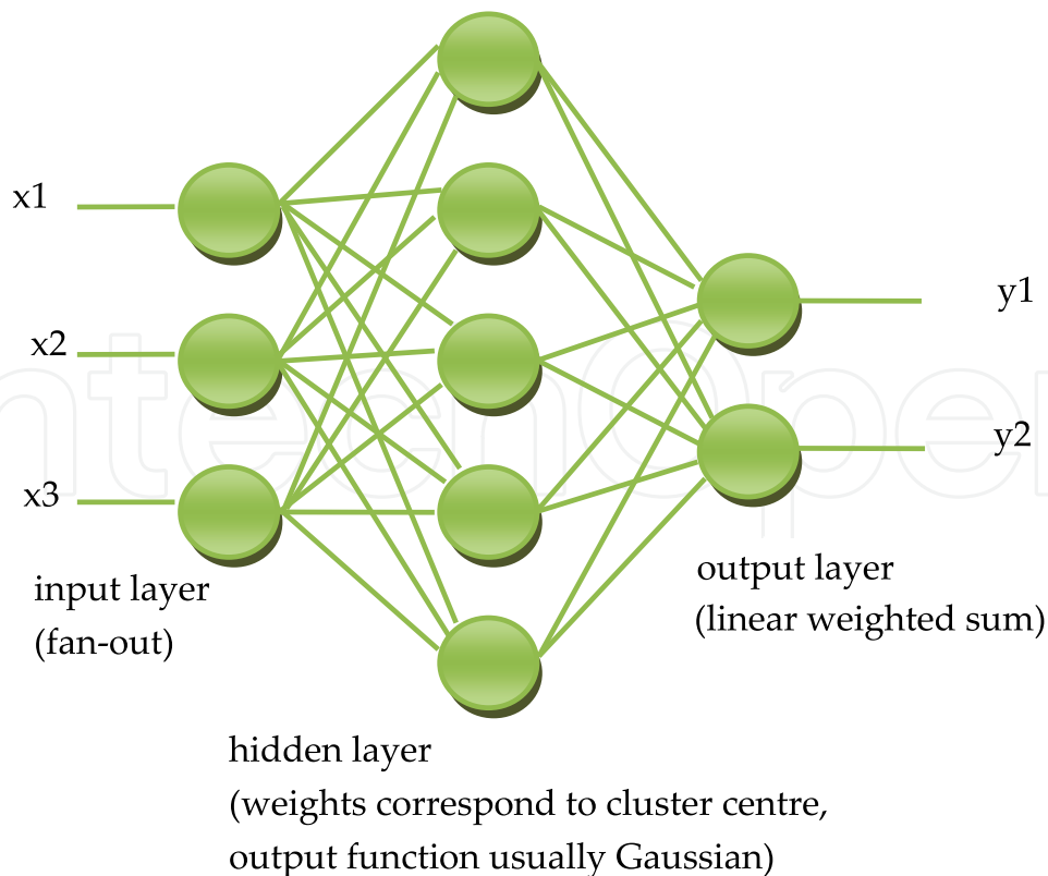
Figure 8. Radial Basis Function Neural Network Architecture
