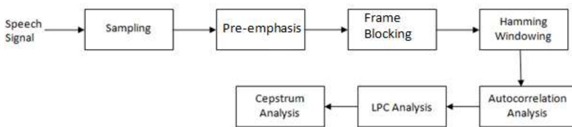
Figure 1. Feature Extractor schematic diagram for LPCC analysis
