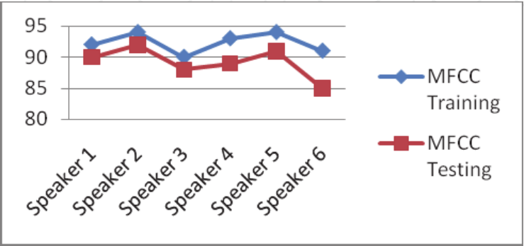
Figure 14. MFCC speaker identification rate with conventional system
