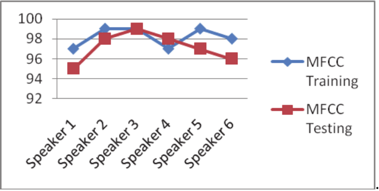
Figure 12. MFCC speaker identification rate with proposed system
