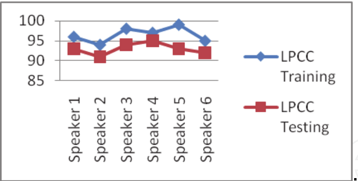
Figure 11. LPCC speaker identification rate with proposed system
