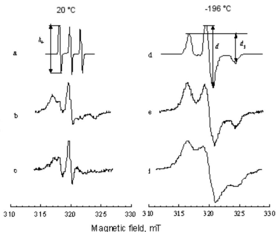
Figure 8. EPR spectra of free 4d in water (a) and ethanol (d), and DNA modified by 4d (b, e), and 3b (c, f) in aqueous 0.01 M NaHCO 3 at Pt-to-nucleotide ratio r = 0.16 , 37°C, 24 h. Spectra were recorded at magnetic modulation 0.32 mT, microwave power 5 (20°C) and 0.5 mW (–196°C), field scan 20 mT, scan time 8 min, time constant 1 s.
