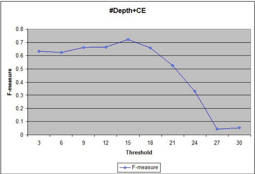
Figure 7. F-measure of the #Depth+CE method ( \beta=0.25 ).
