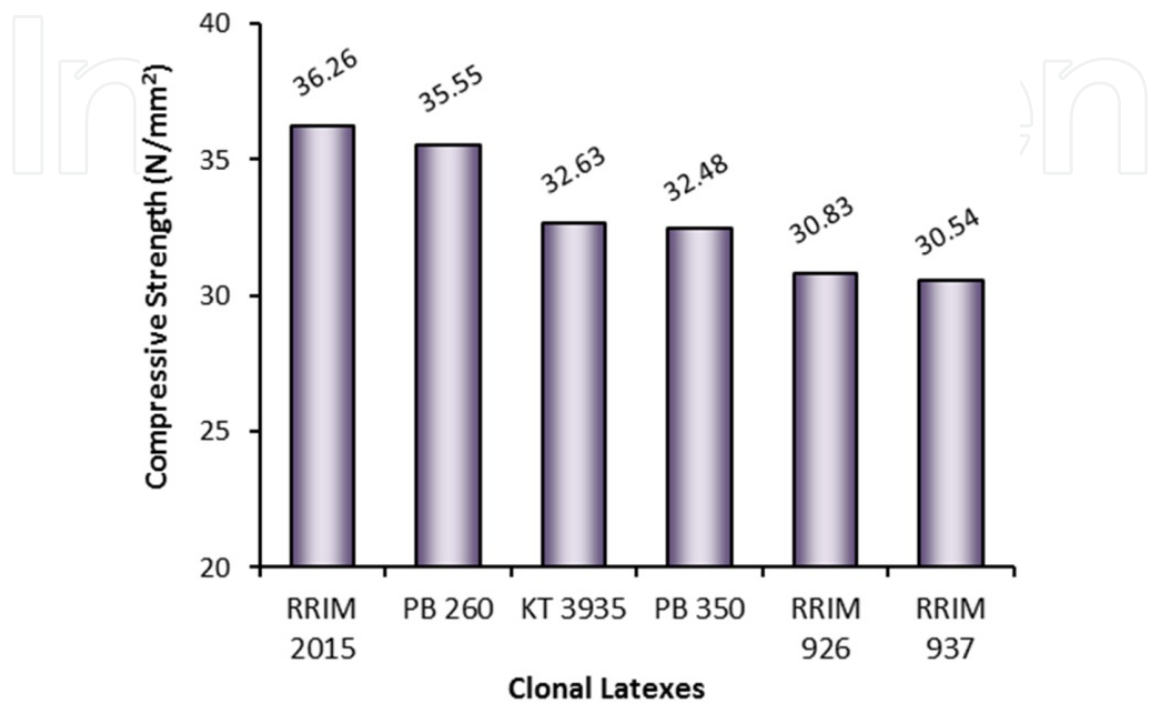
Figure 5. Compressive strength of NRL concrete due to clonal latexes
