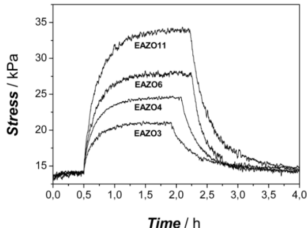
Figure 15. Opto-mechanical experiments for the different nematic liquid single crystal elastomers under irradiation with UV light ( \lambda_{\text{irrad}} = 380 \text{ nm} ) at 333 K (left). Evolution of the maximum opto-mechanical response, \Delta\sigma_{\text{max}} , generated by the different elastomers with the temperature (right).
