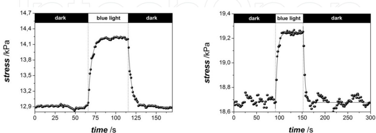
Figure 19. Opto-mechanical experiments for both nematic elastomers EpNO 2 (left) and EoNO 2 (right) at 298 K (irradiation of the networks was performed with blue light, \lambda_{\text{irrad}} = 450\text{ nm} ).
