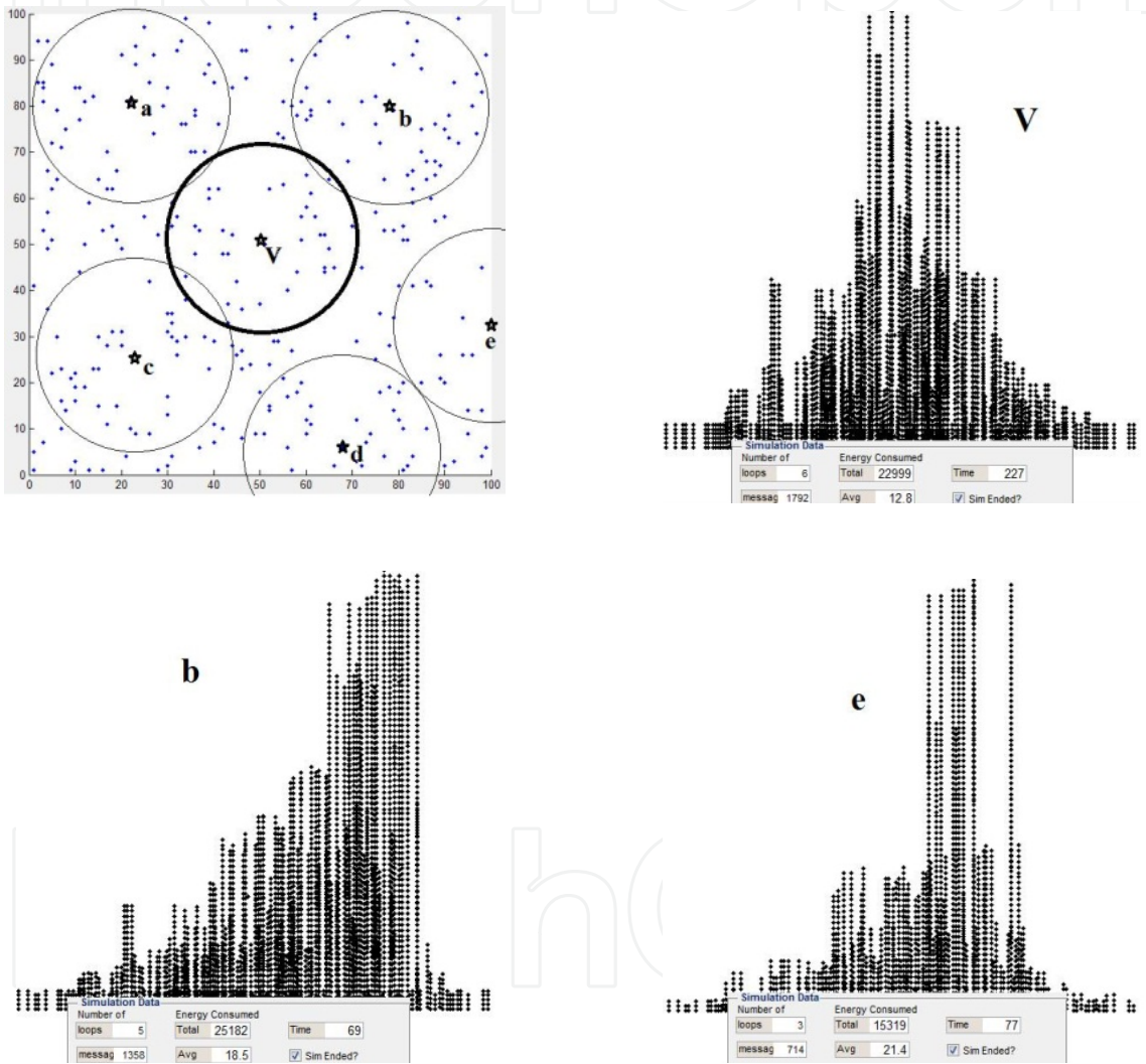
Figure 3. The base station locations and WSN lifespan simulation with energy consumption
